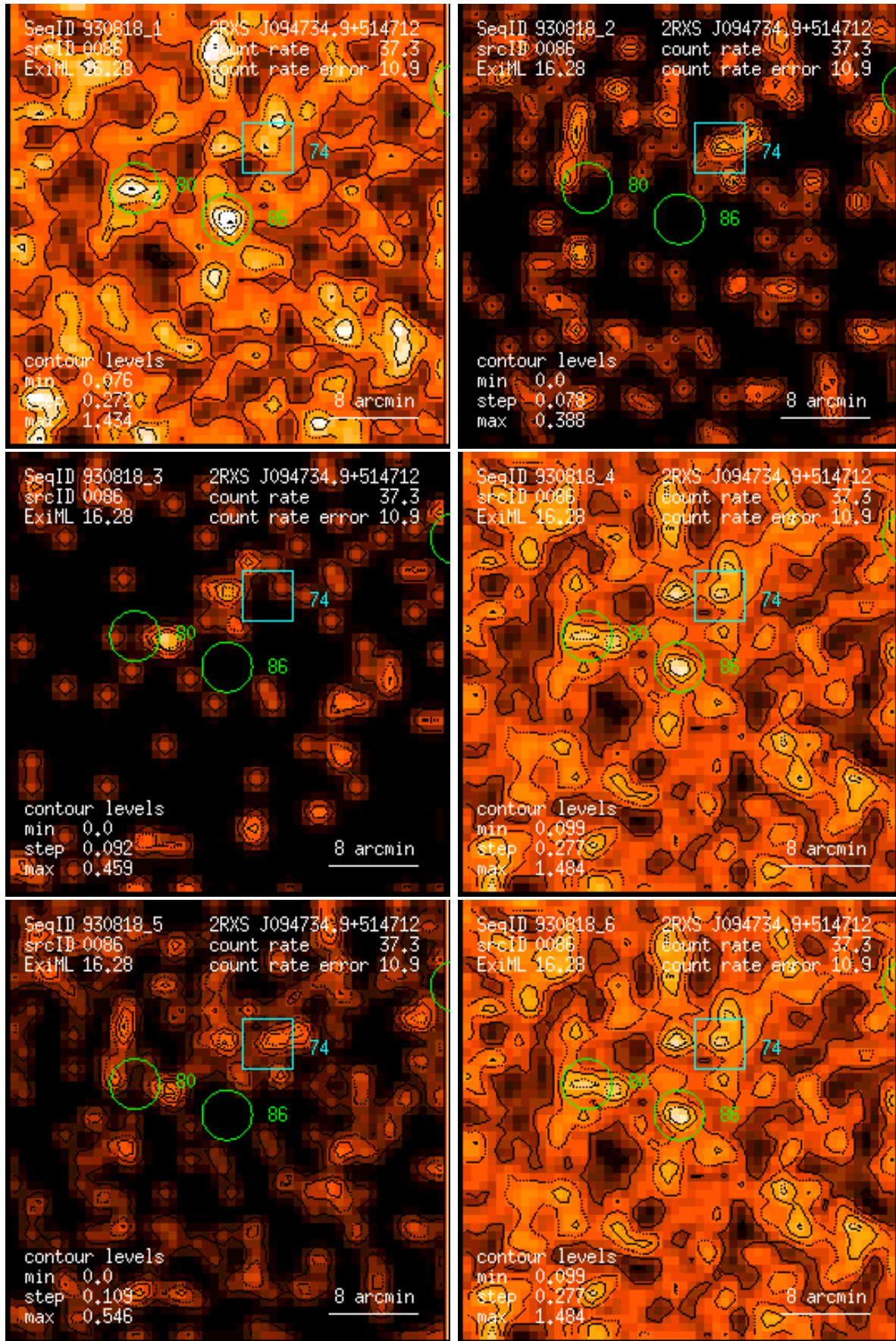
Figure 86: RASS 930818: detection 0086: band rate images, Gaussian filter: (1) PSPC channels 11 – 41, (2) 52 – 90, (3) 91 – 201, (4) 11 – 235, (5) 52 – 201, (6) 11 – 201. Broad band rates in counts/ks. Band rate contour levels in counts/ks/arcmin 2 .
