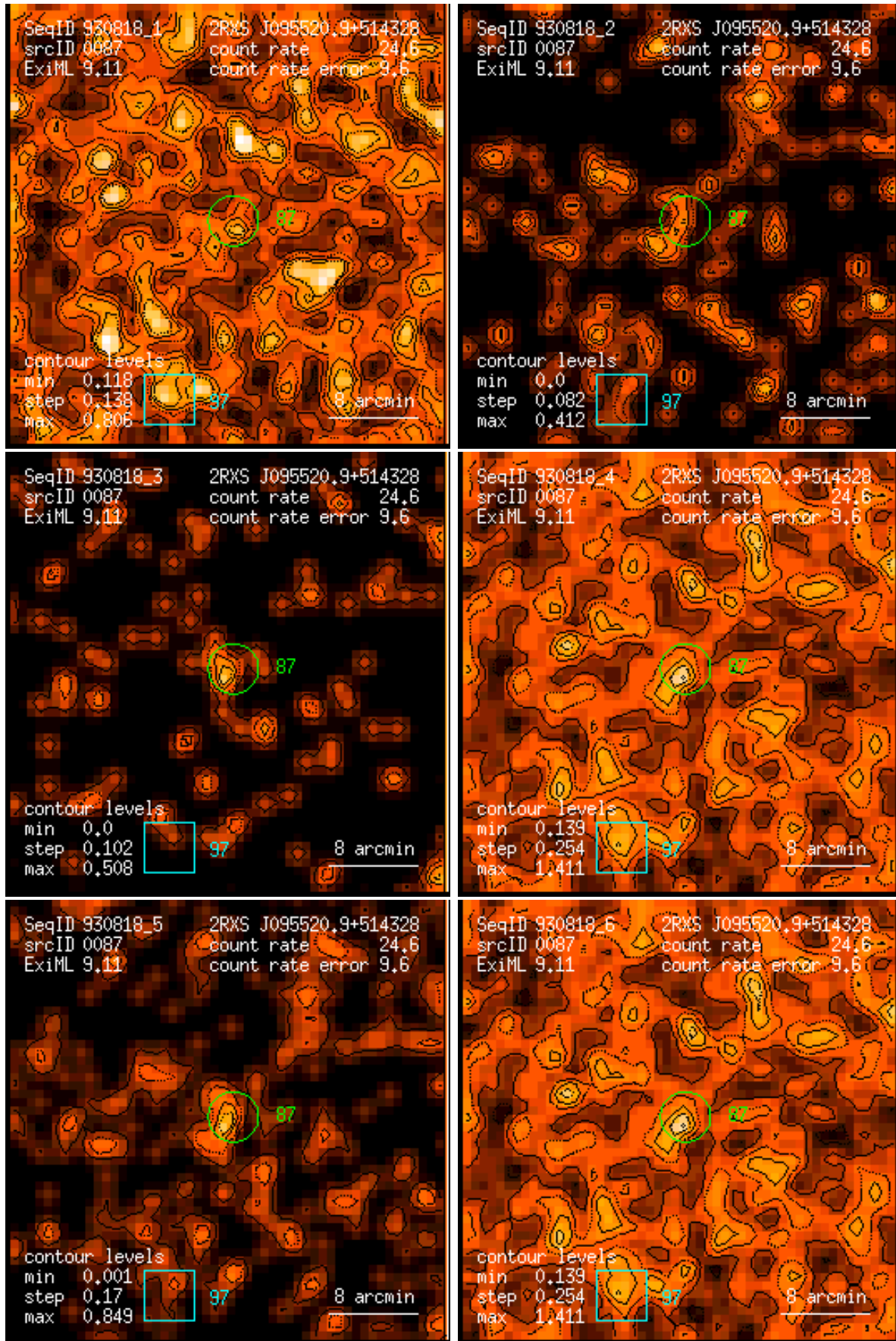
Figure 87: RASS 930818: detection 0087: band rate images, Gaussian filter: (1) PSPC channels 11 – 41, (2) 52 – 90, (3) 91 – 201, (4) 11 – 235, (5) 52 – 201, (6) 11 – 201. Broad band rates in counts/ks. Band rate contour levels in counts/ks/arcmin 2 .
