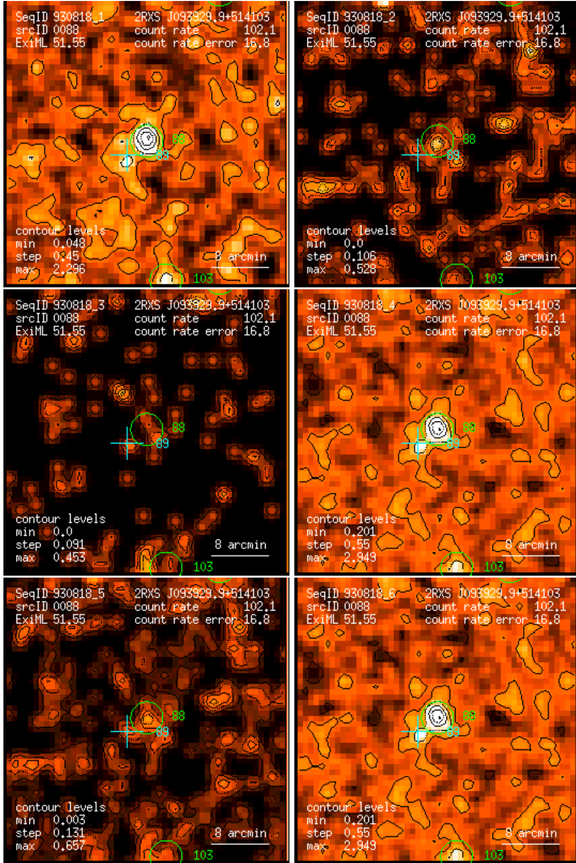
Figure 88: RASS 930818: detection 0088: band rate images, Gaussian filter: (1) PSPC channels 11 – 41, (2) 52 – 90, (3) 91 – 201, (4) 11 – 235, (5) 52 – 201, (6) 11 – 201. Broad band rates in counts/ks. Band rate contour levels in counts/ks/arcmin 2 .
