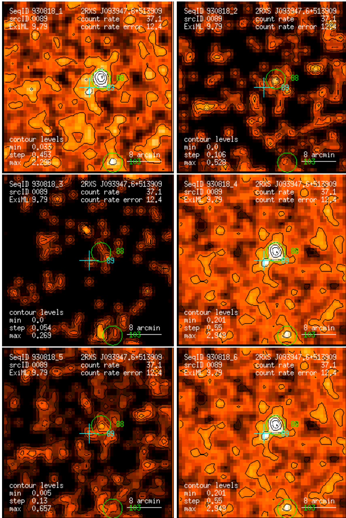
Figure 89: RASS 930818: detection 0089: band rate images, Gaussian filter: (1) PSPC channels 11 – 41, (2) 52 – 90, (3) 91 – 201, (4) 11 – 235, (5) 52 – 201, (6) 11 – 201. Broad band rates in counts/ks. Band rate contour levels in counts/ks/arcmin 2 .
