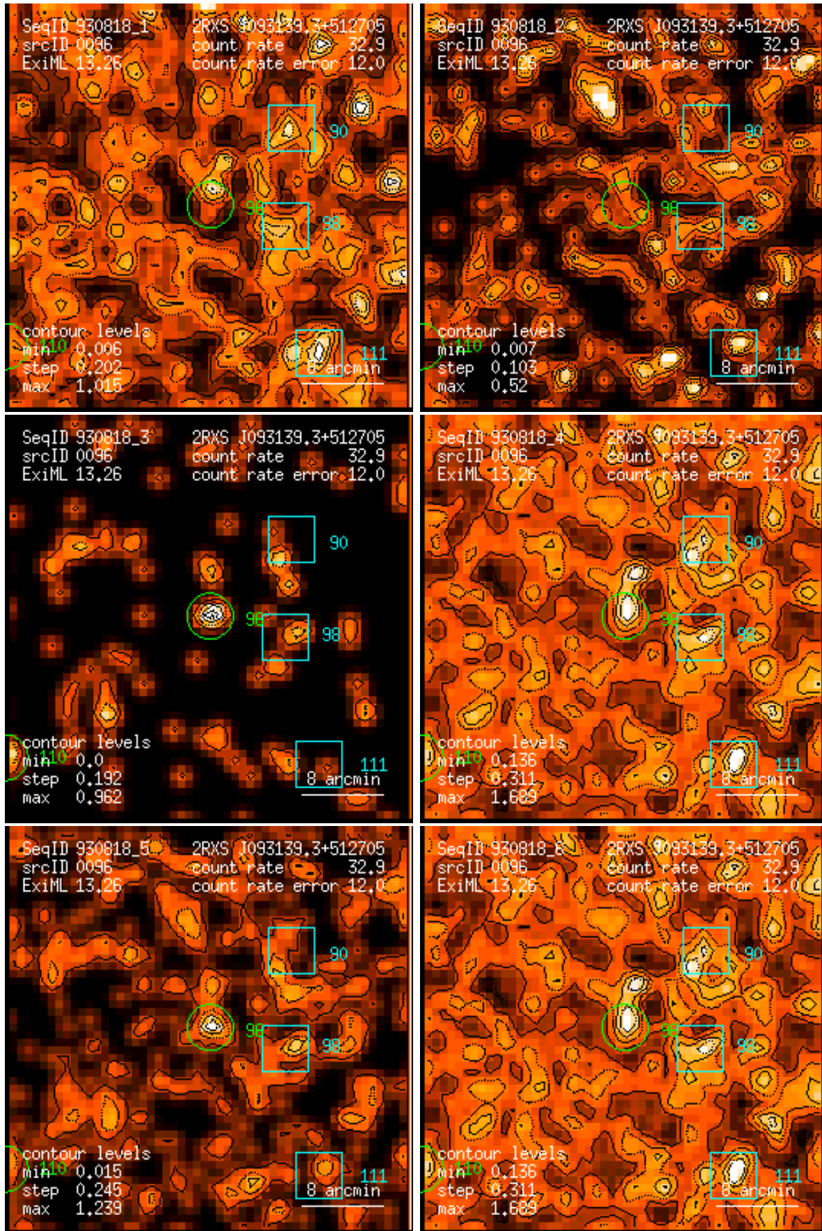
Figure 96: RASS 930818: detection 0096: band rate images, Gaussian filter: (1) PSPC channels 11 – 41, (2) 52 – 90, (3) 91 – 201, (4) 11 – 235, (5) 52 – 201, (6) 11 – 201. Broad band rates in counts/ks. Band rate contour levels in counts/ks/arcmin 2 .
