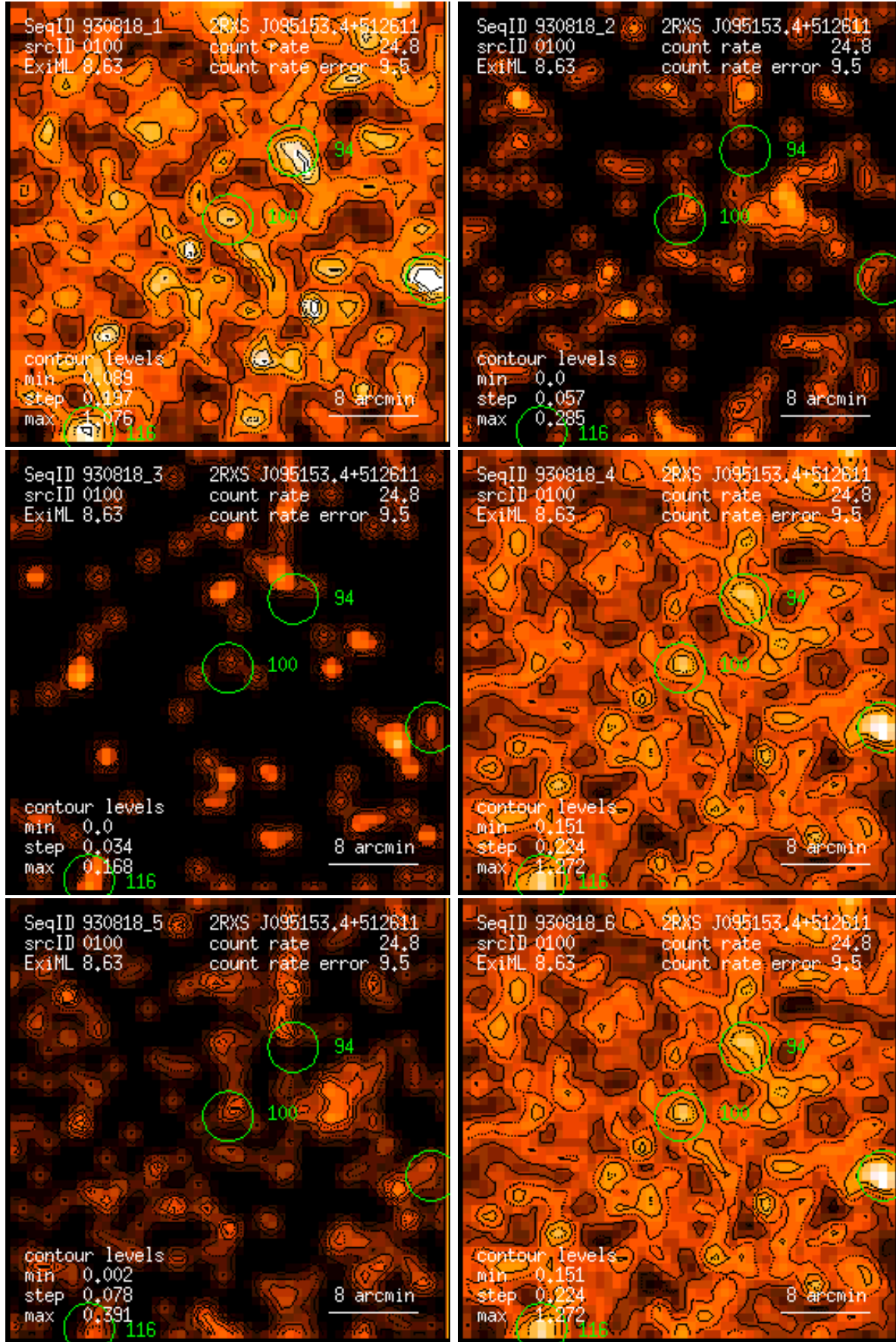
Figure 100: RASS 930818: detection 0100: band rate images, Gaussian filter: (1) PSPC channels 11 – 41, (2) 52 – 90, (3) 91 – 201, (4) 11 – 235, (5) 52 – 201, (6) 11 – 201. Broad band rates in counts/ks. Band rate contour levels in counts/ks/arcmin 2 .
