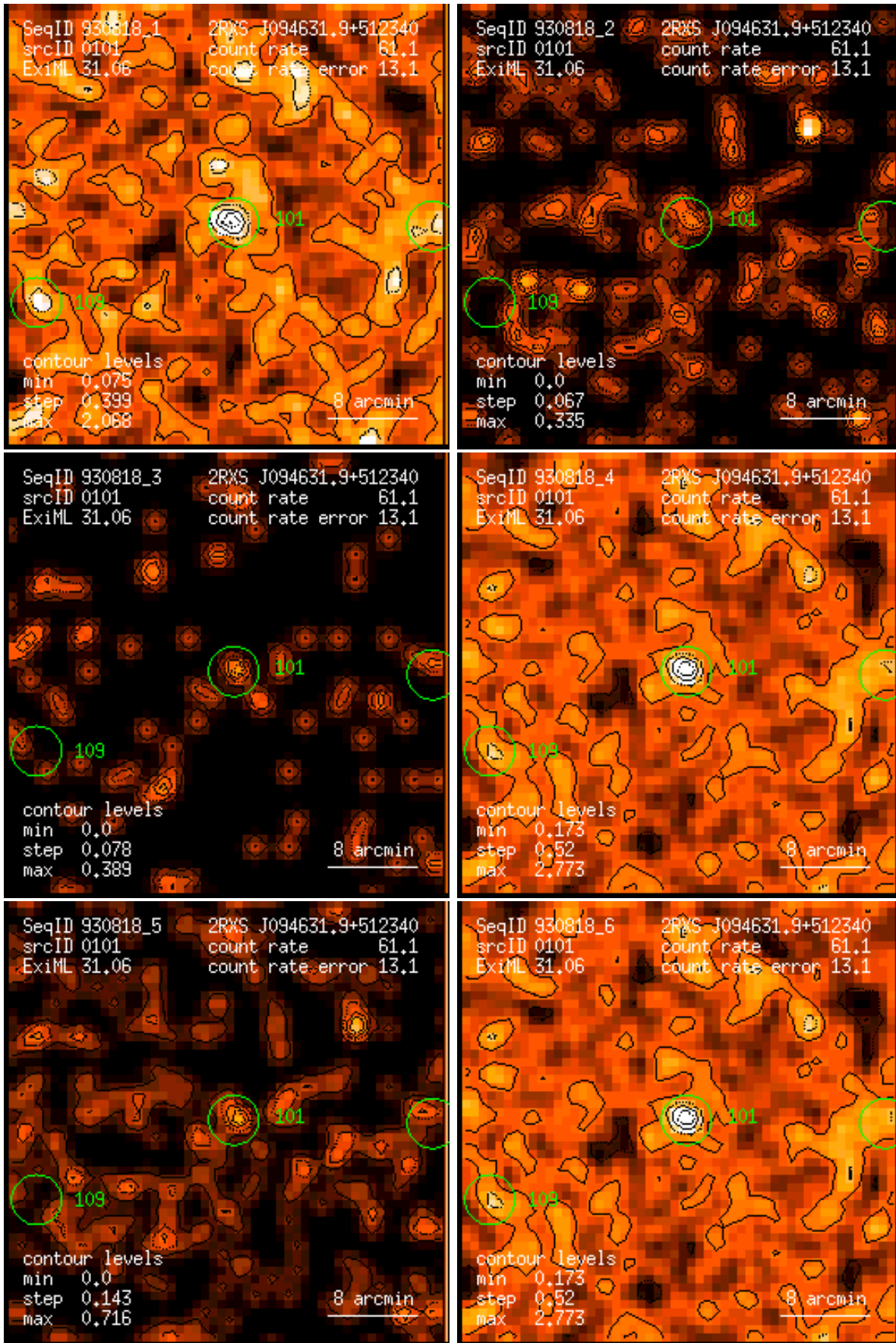
Figure 101: RASS 930818: detection 0101: band rate images, Gaussian filter: (1) PSPC channels 11 – 41, (2) 52 – 90, (3) 91 – 201, (4) 11 – 235, (5) 52 – 201, (6) 11 – 201. Broad band rates in counts/ks. Band rate contour levels in counts/ks/arcmin 2 .
