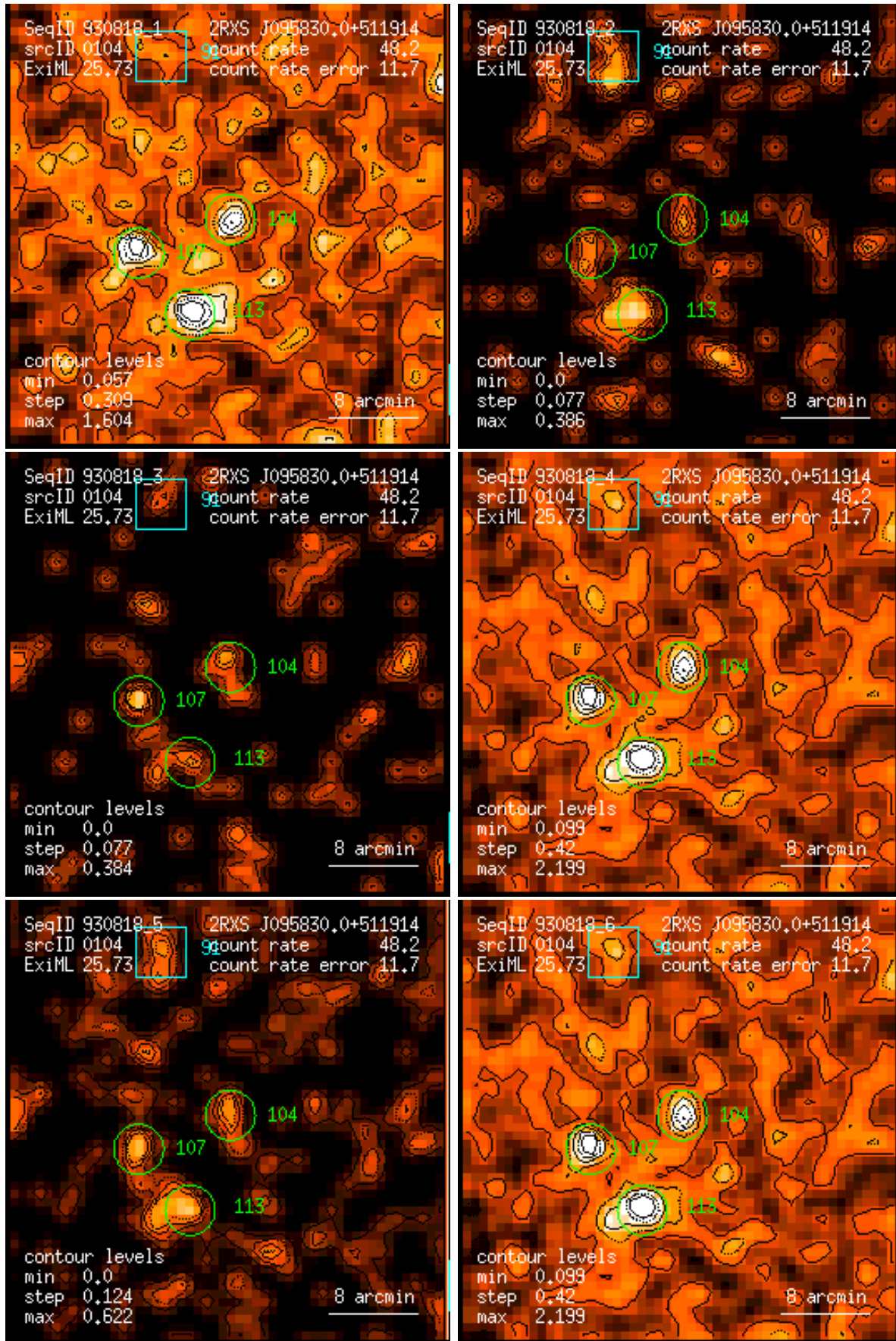
Figure 104: RASS 930818: detection 0104: band rate images, Gaussian filter: (1) PSPC channels 11 – 41, (2) 52 – 90, (3) 91 – 201, (4) 11 – 235, (5) 52 – 201, (6) 11 – 201. Broad band rates in counts/ks. Band rate contour levels in counts/ks/arcmin 2 .
