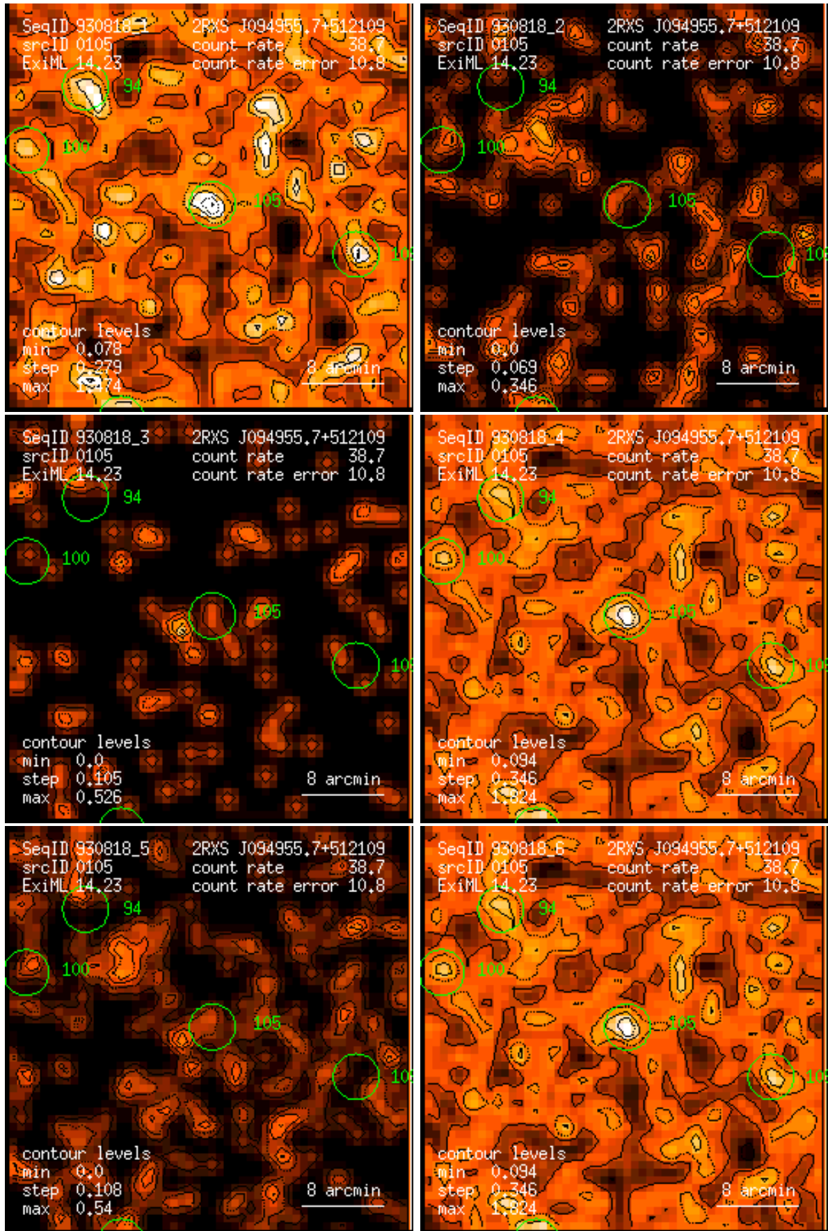
Figure 105: RASS 930818: detection 0105: band rate images, Gaussian filter: (1) PSPC channels 11 – 41, (2) 52 – 90, (3) 91 – 201, (4) 11 – 235, (5) 52 – 201, (6) 11 – 201. Broad band rates in counts/ks. Band rate contour levels in counts/ks/arcmin 2 .
