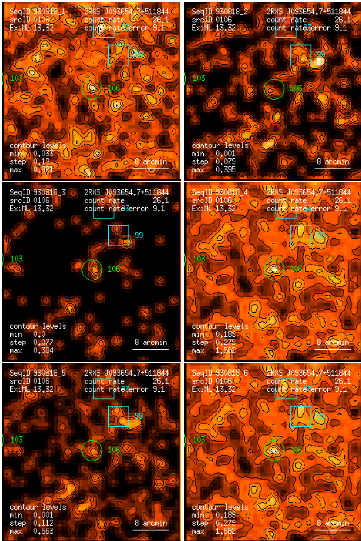
Figure 106: RASS 930818: detection 0106: band rate images, Gaussian filter: (1) PSPC channels 11 – 41, (2) 52 – 90, (3) 91 – 201, (4) 11 – 235, (5) 52 – 201, (6) 11 – 201. Broad band rates in counts/ks. Band rate contour levels in counts/ks/arcmin 2 .
