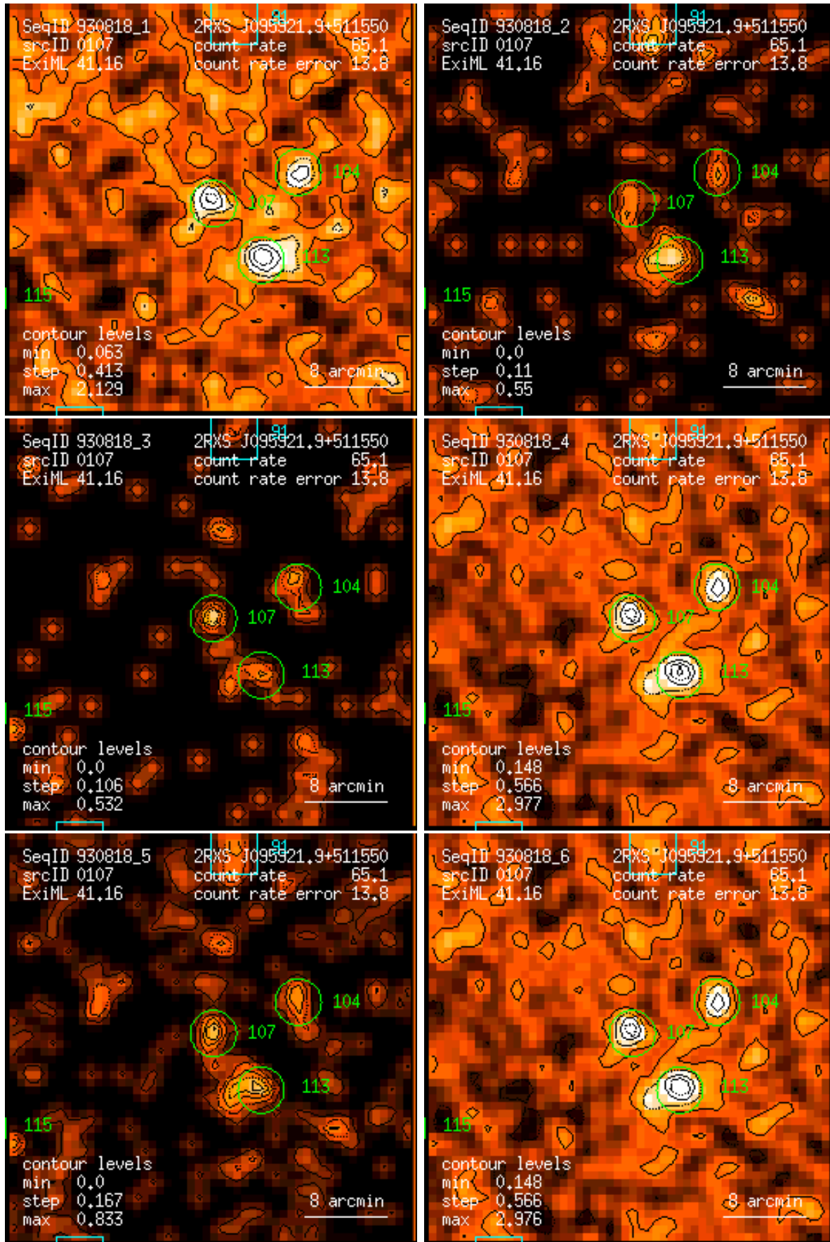
Figure 107: RASS 930818: detection 0107: band rate images, Gaussian filter: (1) PSPC channels 11 – 41, (2) 52 – 90, (3) 91 – 201, (4) 11 – 235, (5) 52 – 201, (6) 11 – 201. Broad band rates in counts/ks. Band rate contour levels in counts/ks/arcmin 2 .
