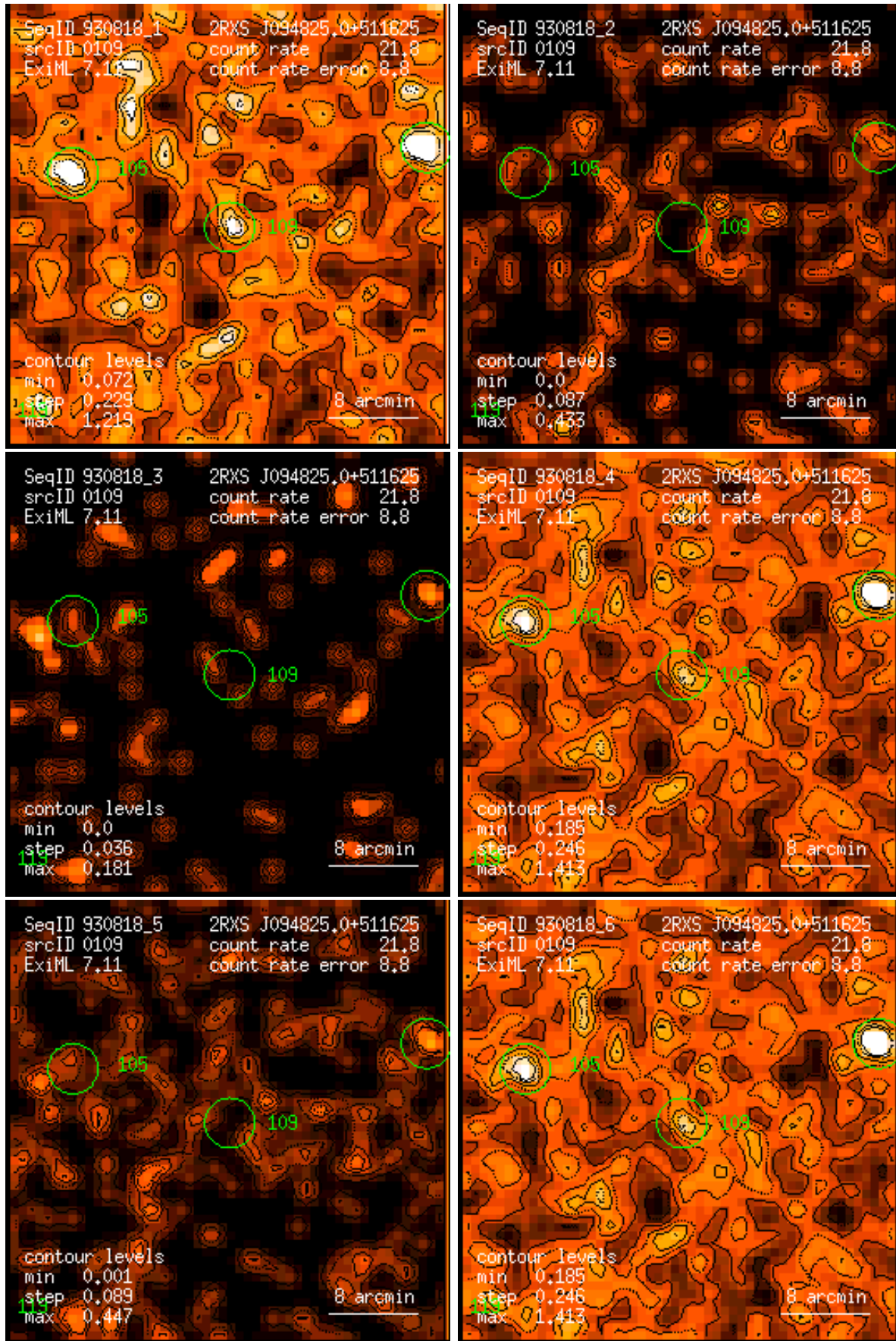
Figure 109: RASS 930818: detection 0109: band rate images, Gaussian filter: (1) PSPC channels 11 – 41, (2) 52 – 90, (3) 91 – 201, (4) 11 – 235, (5) 52 – 201, (6) 11 – 201. Broad band rates in counts/ks. Band rate contour levels in counts/ks/arcmin 2 .
