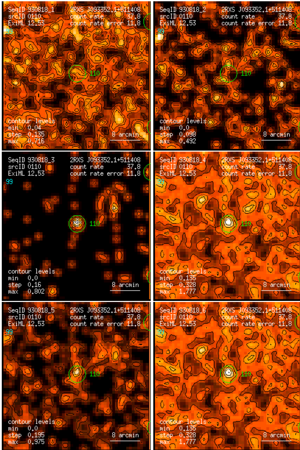
Figure 110: RASS 930818: detection 0110: band rate images, Gaussian filter: (1) PSPC channels 11 – 41, (2) 52 – 90, (3) 91 – 201, (4) 11 – 235, (5) 52 – 201, (6) 11 – 201. Broad band rates in counts/ks. Band rate contour levels in counts/ks/arcmin 2 .
