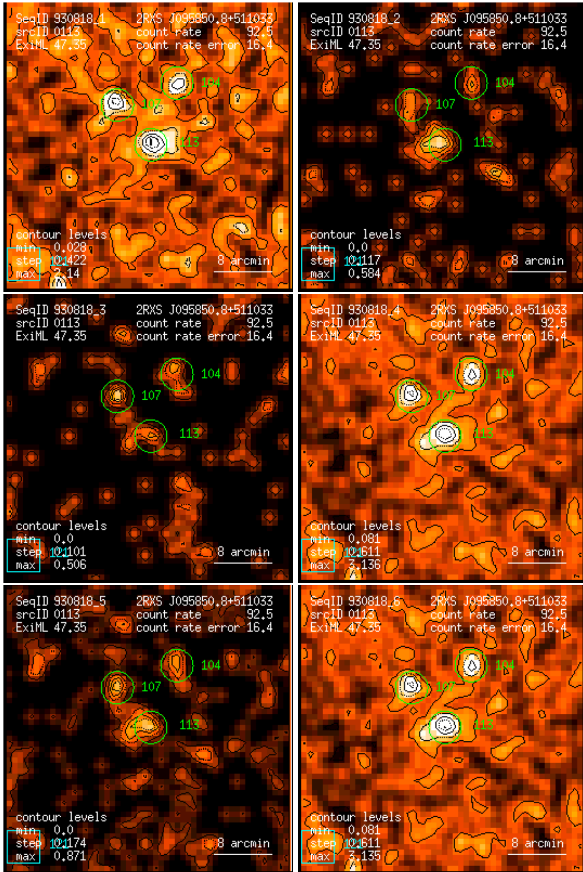
Figure 113: RASS 930818: detection 0113: band rate images, Gaussian filter: (1) PSPC channels 11 – 41, (2) 52 – 90, (3) 91 – 201, (4) 11 – 235, (5) 52 – 201, (6) 11 – 201. Broad band rates in counts/ks. Band rate contour levels in counts/ks/arcmin 2 .
