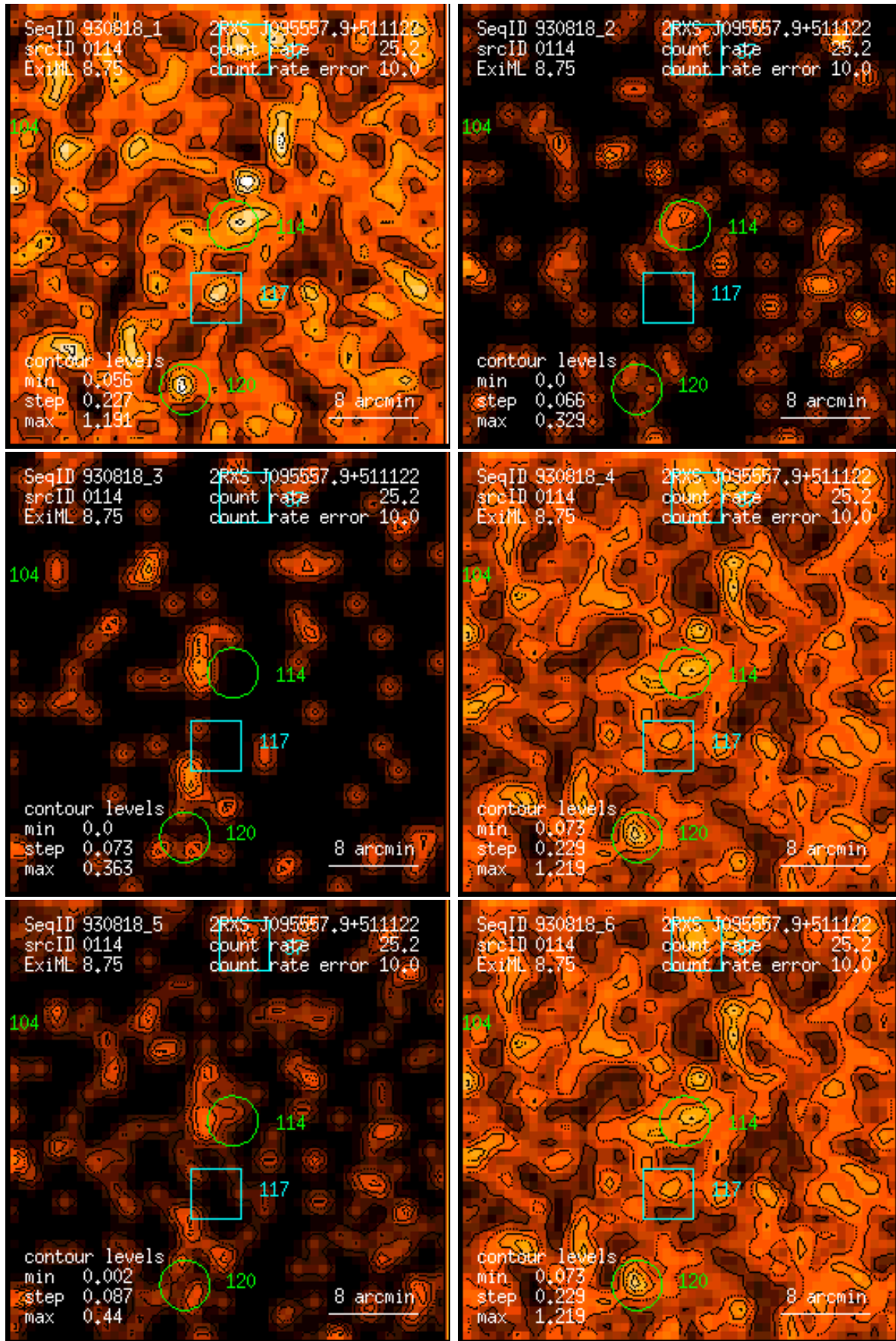
Figure 114: RASS 930818: detection 0114: band rate images, Gaussian filter: (1) PSPC channels 11 – 41, (2) 52 – 90, (3) 91 – 201, (4) 11 – 235, (5) 52 – 201, (6) 11 – 201. Broad band rates in counts/ks. Band rate contour levels in counts/ks/arcmin 2 .
