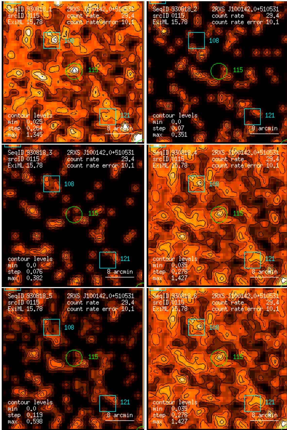
Figure 115: RASS 930818: detection 0115: band rate images, Gaussian filter: (1) PSPC channels 11 – 41, (2) 52 – 90, (3) 91 – 201, (4) 11 – 235, (5) 52 – 201, (6) 11 – 201. Broad band rates in counts/ks. Band rate contour levels in counts/ks/arcmin 2 .
