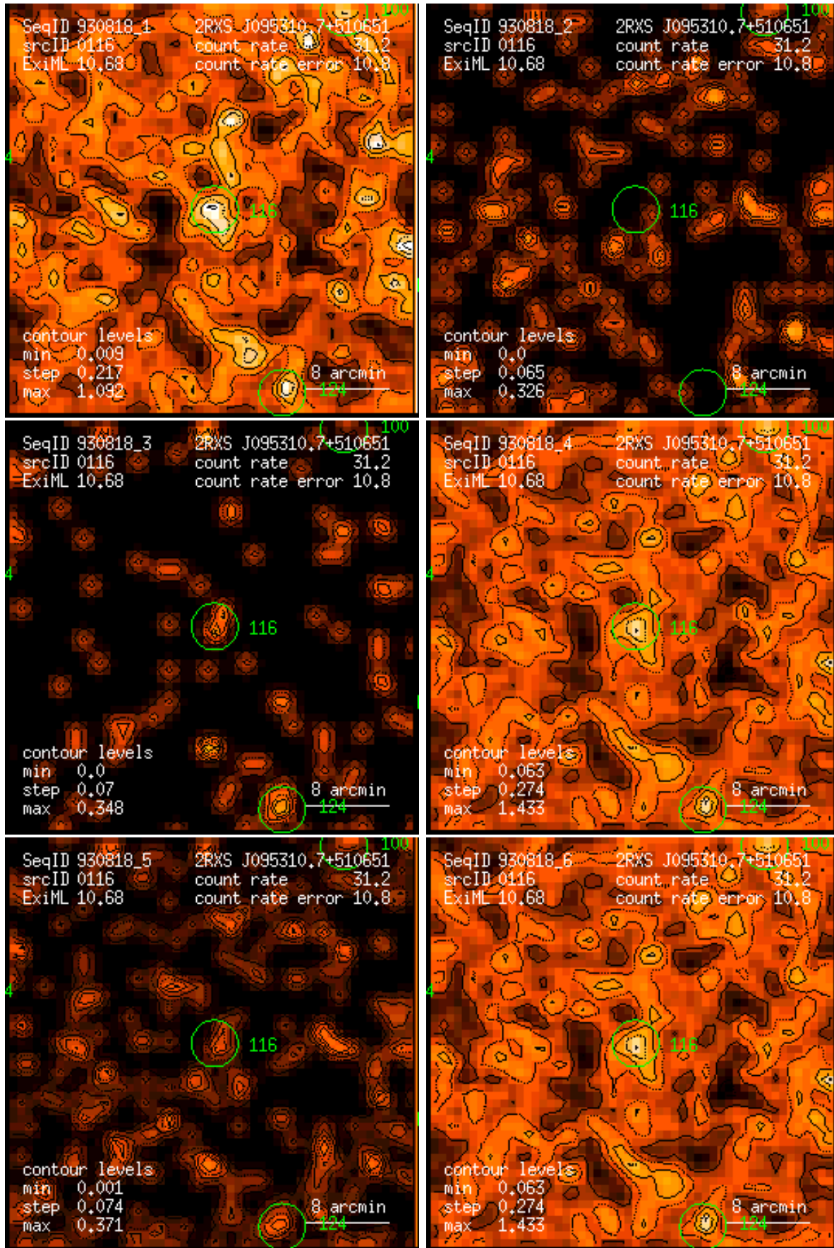
Figure 116: RASS 930818: detection 0116: band rate images, Gaussian filter: (1) PSPC channels 11 – 41, (2) 52 – 90, (3) 91 – 201, (4) 11 – 235, (5) 52 – 201, (6) 11 – 201. Broad band rates in counts/ks. Band rate contour levels in counts/ks/arcmin 2 .
