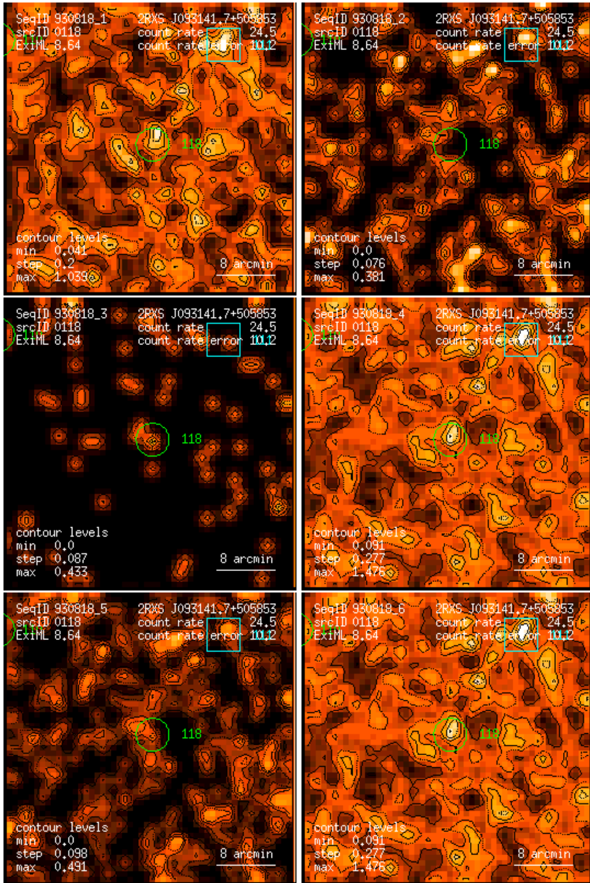
Figure 118: RASS 930818: detection 0118: band rate images, Gaussian filter: (1) PSPC channels 11 – 41, (2) 52 – 90, (3) 91 – 201, (4) 11 – 235, (5) 52 – 201, (6) 11 – 201. Broad band rates in counts/ks. Band rate contour levels in counts/ks/arcmin 2 .
