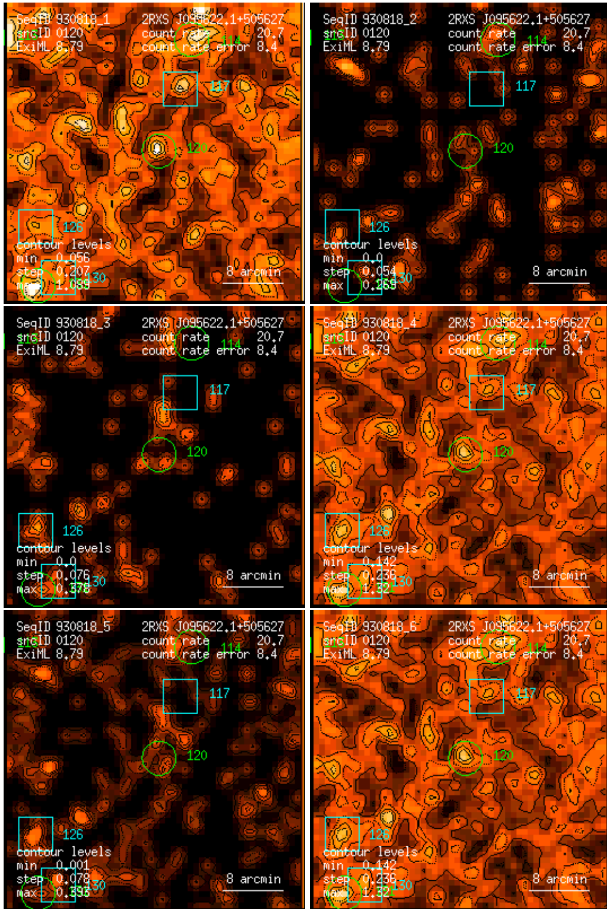
Figure 120: RASS 930818: detection 0120: band rate images, Gaussian filter: (1) PSPC channels 11 – 41, (2) 52 – 90, (3) 91 – 201, (4) 11 – 235, (5) 52 – 201, (6) 11 – 201. Broad band rates in counts/ks. Band rate contour levels in counts/ks/arcmin 2 .
