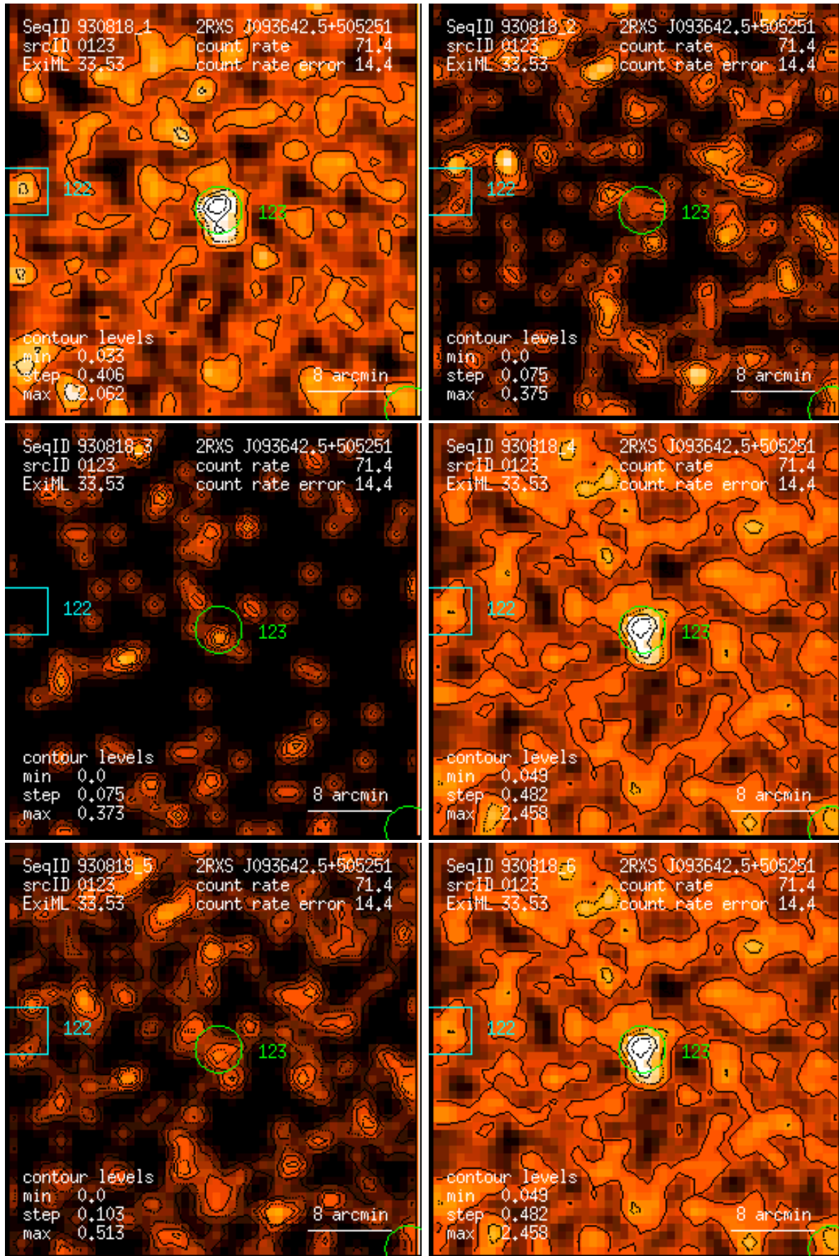
Figure 123: RASS 930818: detection 0123: band rate images, Gaussian filter: (1) PSPC channels 11 – 41, (2) 52 – 90, (3) 91 – 201, (4) 11 – 235, (5) 52 – 201, (6) 11 – 201. Broad band rates in counts/ks. Band rate contour levels in counts/ks/arcmin 2 .
