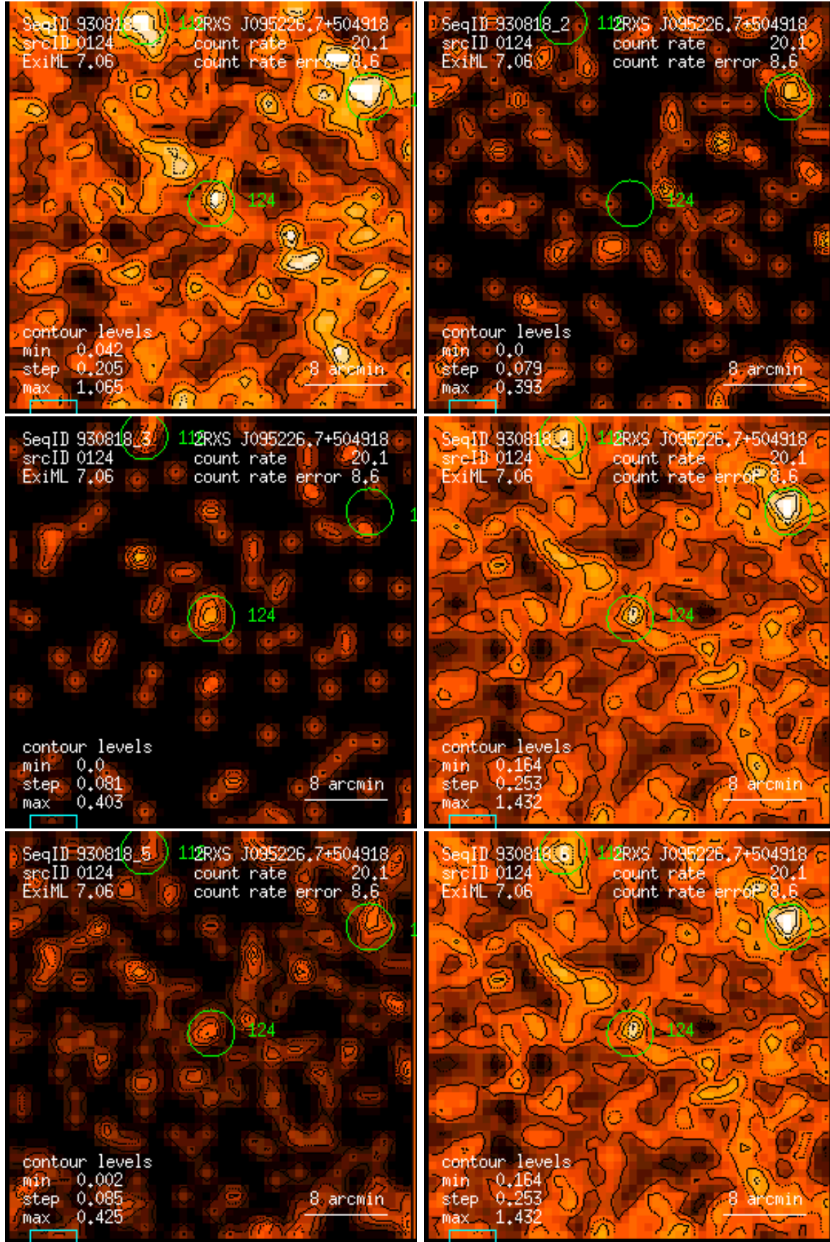
Figure 124: RASS 930818: detection 0124: band rate images, Gaussian filter: (1) PSPC channels 11 – 41, (2) 52 – 90, (3) 91 – 201, (4) 11 – 235, (5) 52 – 201, (6) 11 – 201. Broad band rates in counts/ks. Band rate contour levels in counts/ks/arcmin 2 .
