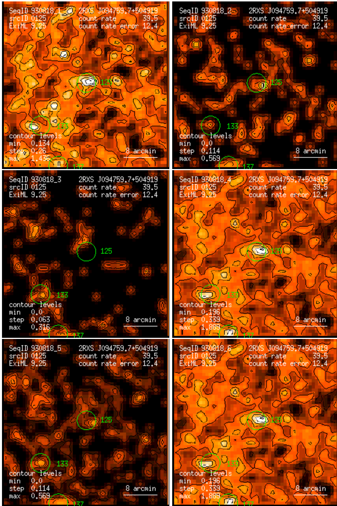
Figure 125: RASS 930818: detection 0125: band rate images, Gaussian filter: (1) PSPC channels 11 – 41, (2) 52 – 90, (3) 91 – 201, (4) 11 – 235, (5) 52 – 201, (6) 11 – 201. Broad band rates in counts/ks. Band rate contour levels in counts/ks/arcmin 2 .
