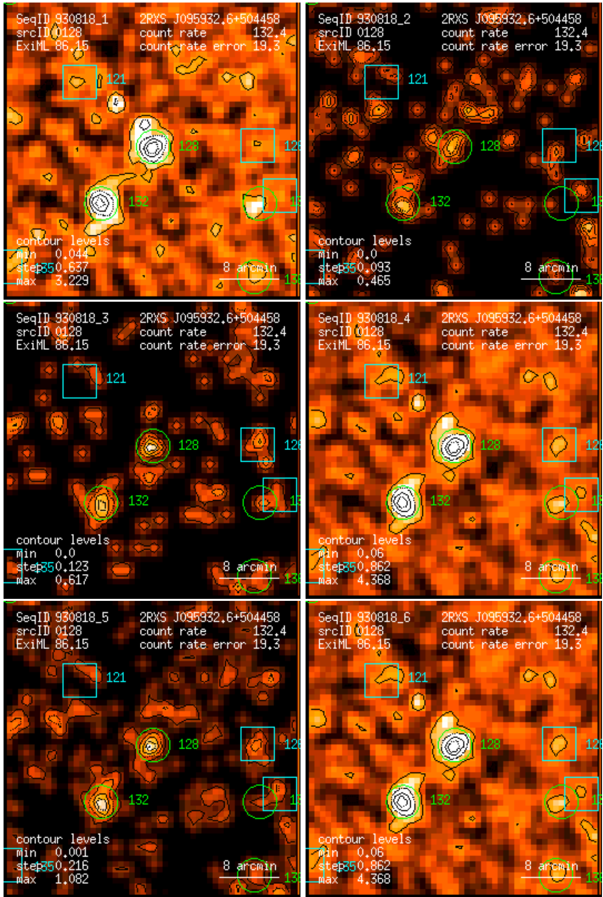
Figure 128: RASS 930818: detection 0128: band rate images, Gaussian filter: (1) PSPC channels 11 – 41, (2) 52 – 90, (3) 91 – 201, (4) 11 – 235, (5) 52 – 201, (6) 11 – 201. Broad band rates in counts/ks. Band rate contour levels in counts/ks/arcmin 2 .
