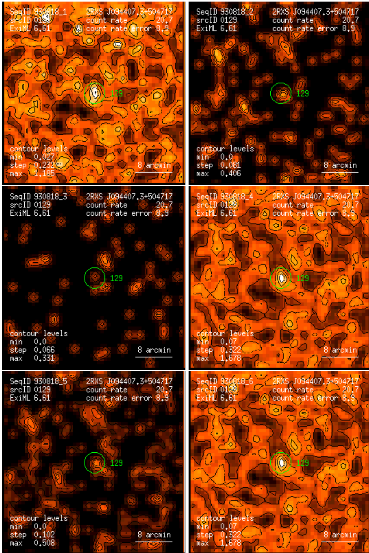
Figure 129: RASS 930818: detection 0129: band rate images, Gaussian filter: (1) PSPC channels 11 – 41, (2) 52 – 90, (3) 91 – 201, (4) 11 – 235, (5) 52 – 201, (6) 11 – 201. Broad band rates in counts/ks. Band rate contour levels in counts/ks/arcmin 2 .
