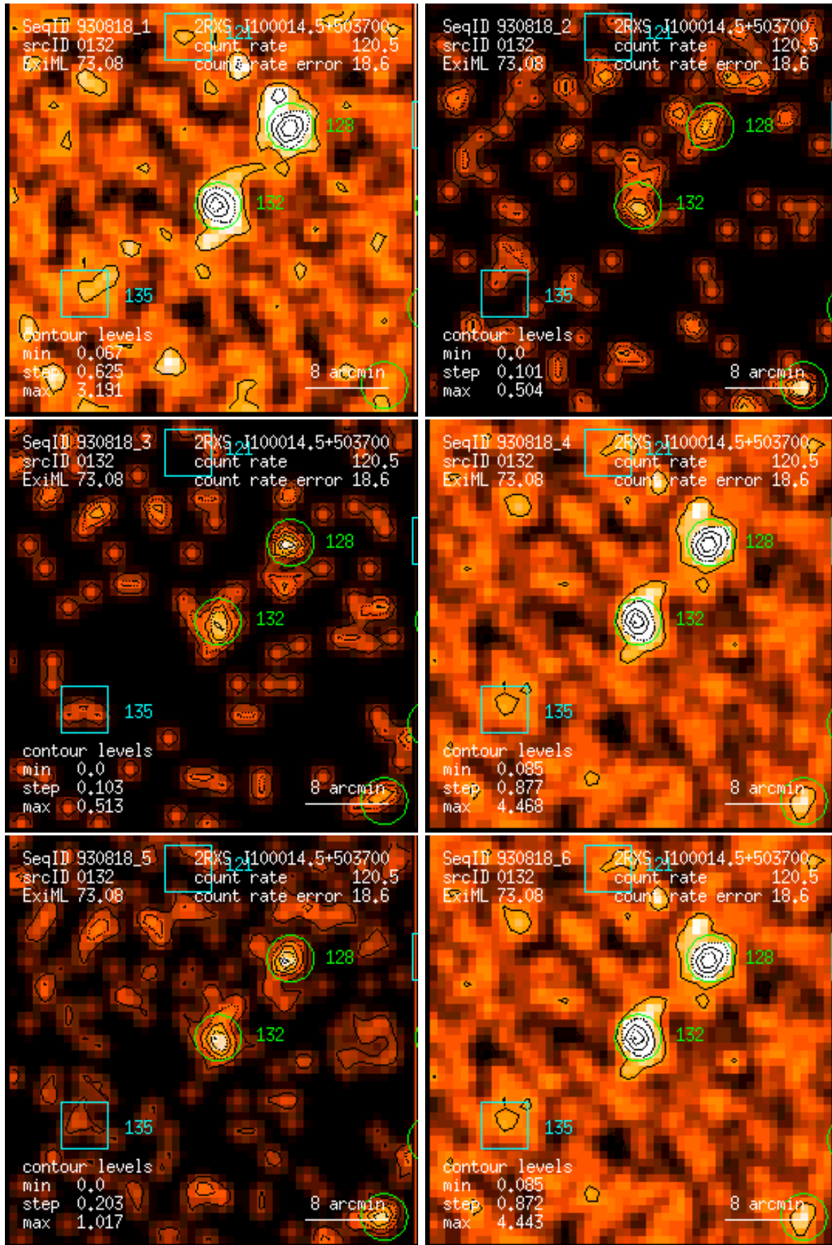
Figure 132: RASS 930818: detection 0132: band rate images, Gaussian filter: (1) PSPC channels 11 – 41, (2) 52 – 90, (3) 91 – 201, (4) 11 – 235, (5) 52 – 201, (6) 11 – 201. Broad band rates in counts/ks. Band rate contour levels in counts/ks/arcmin 2 .
