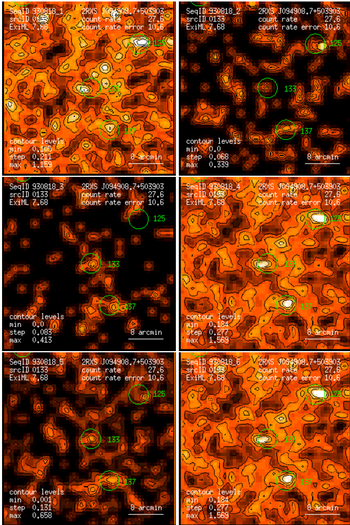
Figure 133: RASS 930818: detection 0133: band rate images, Gaussian filter: (1) PSPC channels 11 – 41, (2) 52 – 90, (3) 91 – 201, (4) 11 – 235, (5) 52 – 201, (6) 11 – 201. Broad band rates in counts/ks. Band rate contour levels in counts/ks/arcmin 2 .
