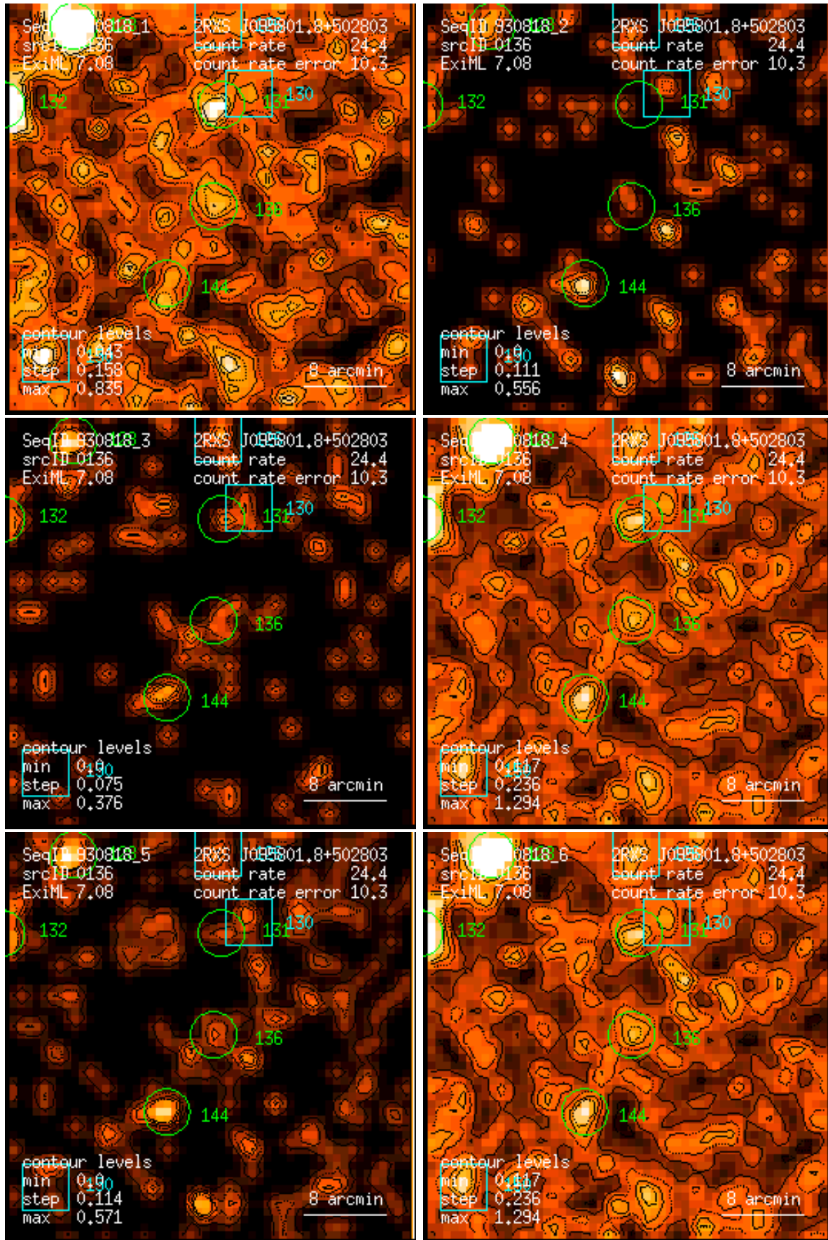
Figure 136: RASS 930818: detection 0136: band rate images, Gaussian filter: (1) PSPC channels 11 – 41, (2) 52 – 90, (3) 91 – 201, (4) 11 – 235, (5) 52 – 201, (6) 11 – 201. Broad band rates in counts/ks. Band rate contour levels in counts/ks/arcmin 2 .
