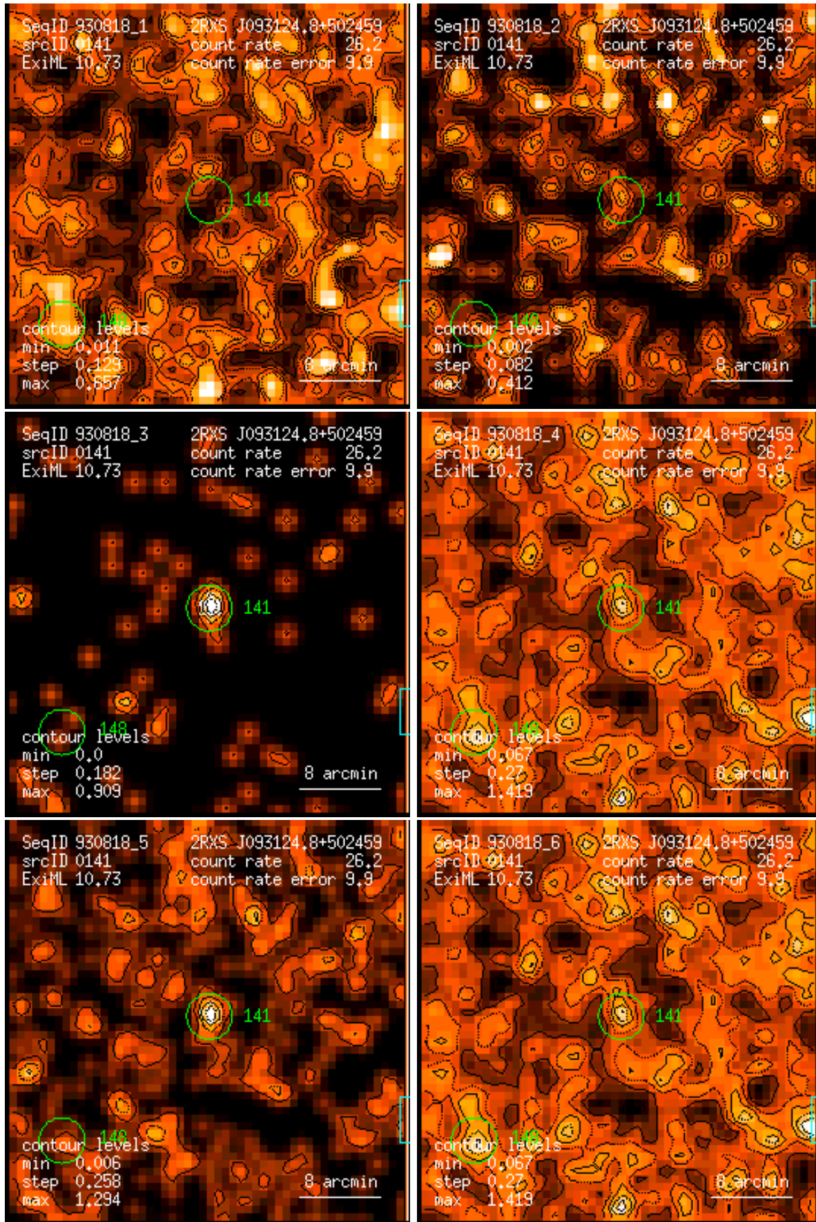
Figure 141: RASS 930818: detection 0141: band rate images, Gaussian filter: (1) PSPC channels 11 – 41, (2) 52 – 90, (3) 91 – 201, (4) 11 – 235, (5) 52 – 201, (6) 11 – 201. Broad band rates in counts/ks. Band rate contour levels in counts/ks/arcmin 2 .
