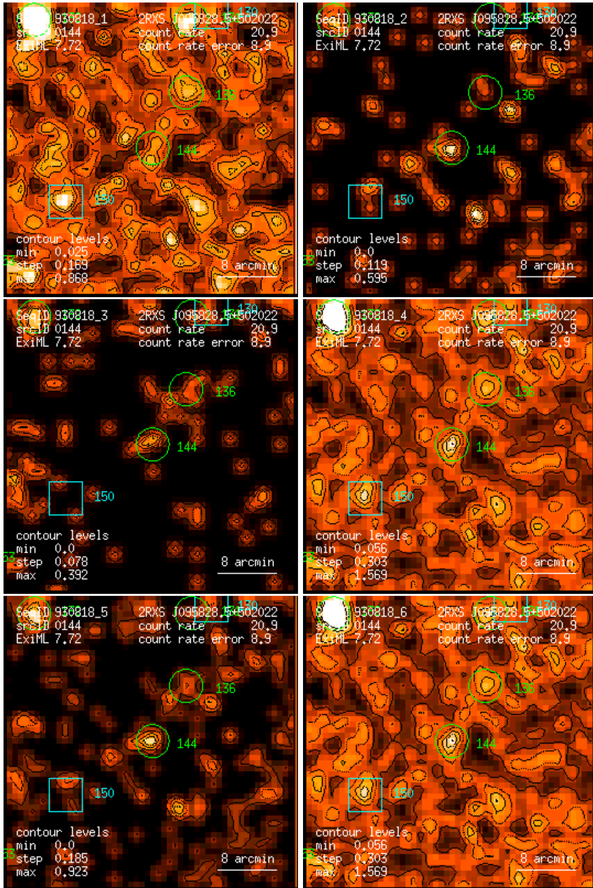
Figure 144: RASS 930818: detection 0144: band rate images, Gaussian filter: (1) PSPC channels 11 – 41, (2) 52 – 90, (3) 91 – 201, (4) 11 – 235, (5) 52 – 201, (6) 11 – 201. Broad band rates in counts/ks. Band rate contour levels in counts/ks/arcmin 2 .
