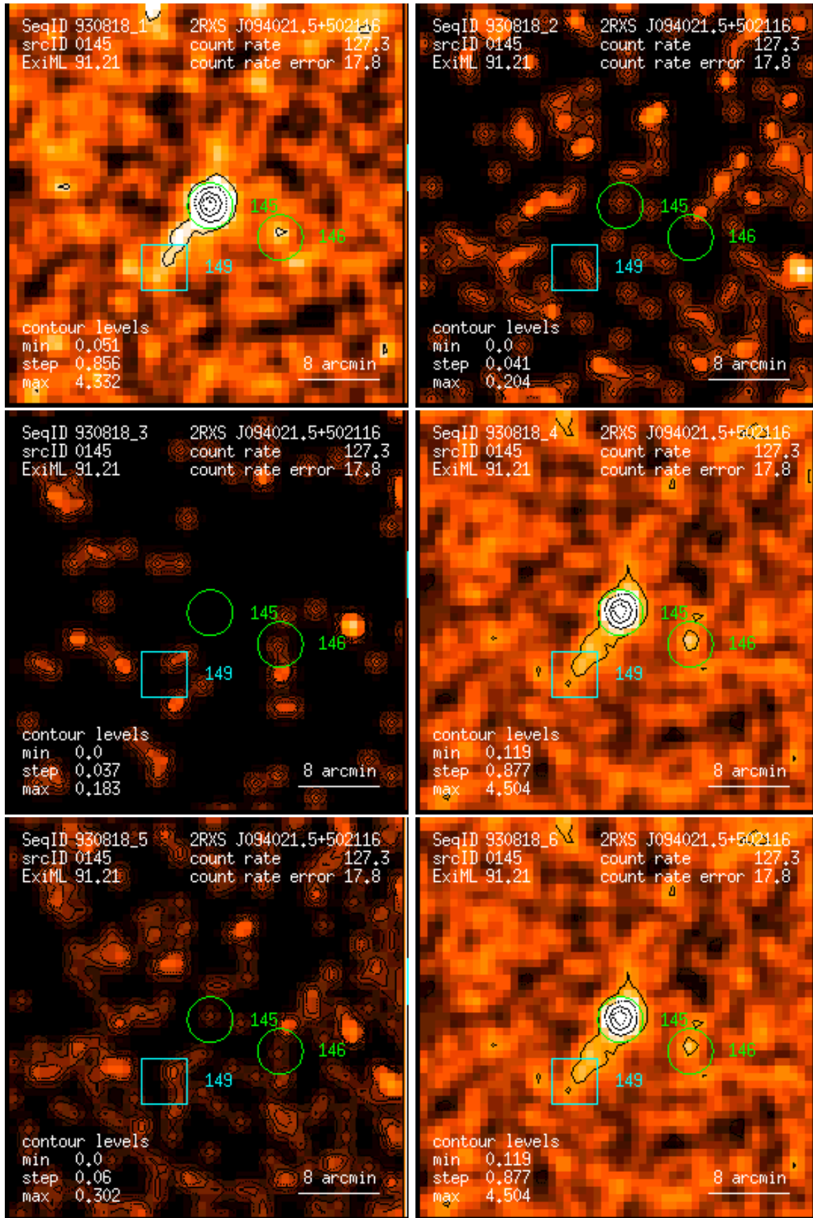
Figure 145: RASS 930818: detection 0145: band rate images, Gaussian filter: (1) PSPC channels 11 – 41, (2) 52 – 90, (3) 91 – 201, (4) 11 – 235, (5) 52 – 201, (6) 11 – 201. Broad band rates in counts/ks. Band rate contour levels in counts/ks/arcmin 2 .
