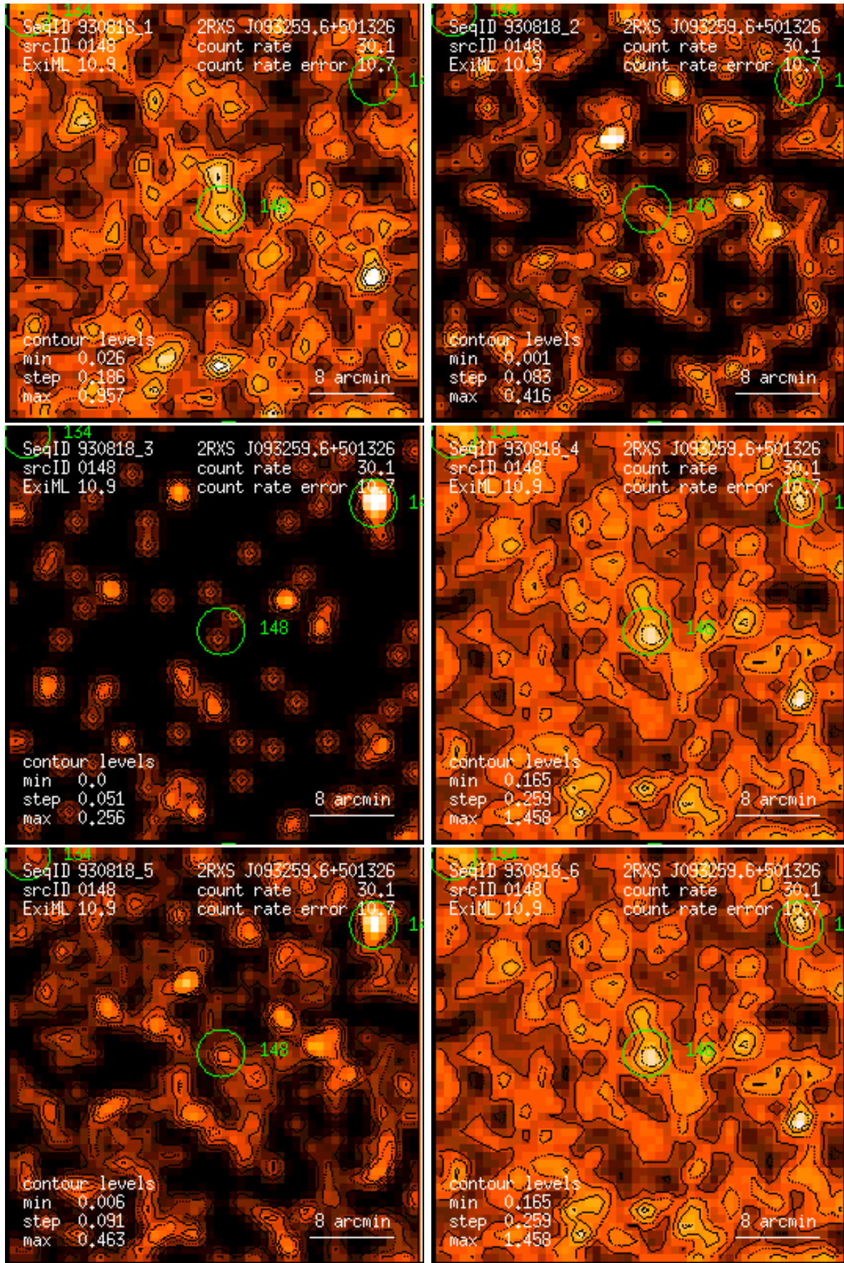
Figure 148: RASS 930818: detection 0148: band rate images, Gaussian filter: (1) PSPC channels 11 – 41, (2) 52 – 90, (3) 91 – 201, (4) 11 – 235, (5) 52 – 201, (6) 11 – 201. Broad band rates in counts/ks. Band rate contour levels in counts/ks/arcmin 2 .
