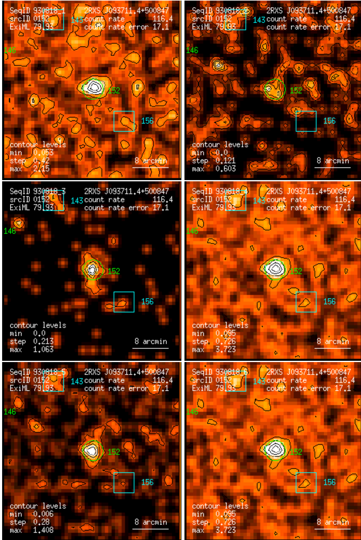
Figure 152: RASS 930818: detection 0152: band rate images, Gaussian filter: (1) PSPC channels 11 – 41, (2) 52 – 90, (3) 91 – 201, (4) 11 – 235, (5) 52 – 201, (6) 11 – 201. Broad band rates in counts/ks. Band rate contour levels in counts/ks/arcmin 2 .
