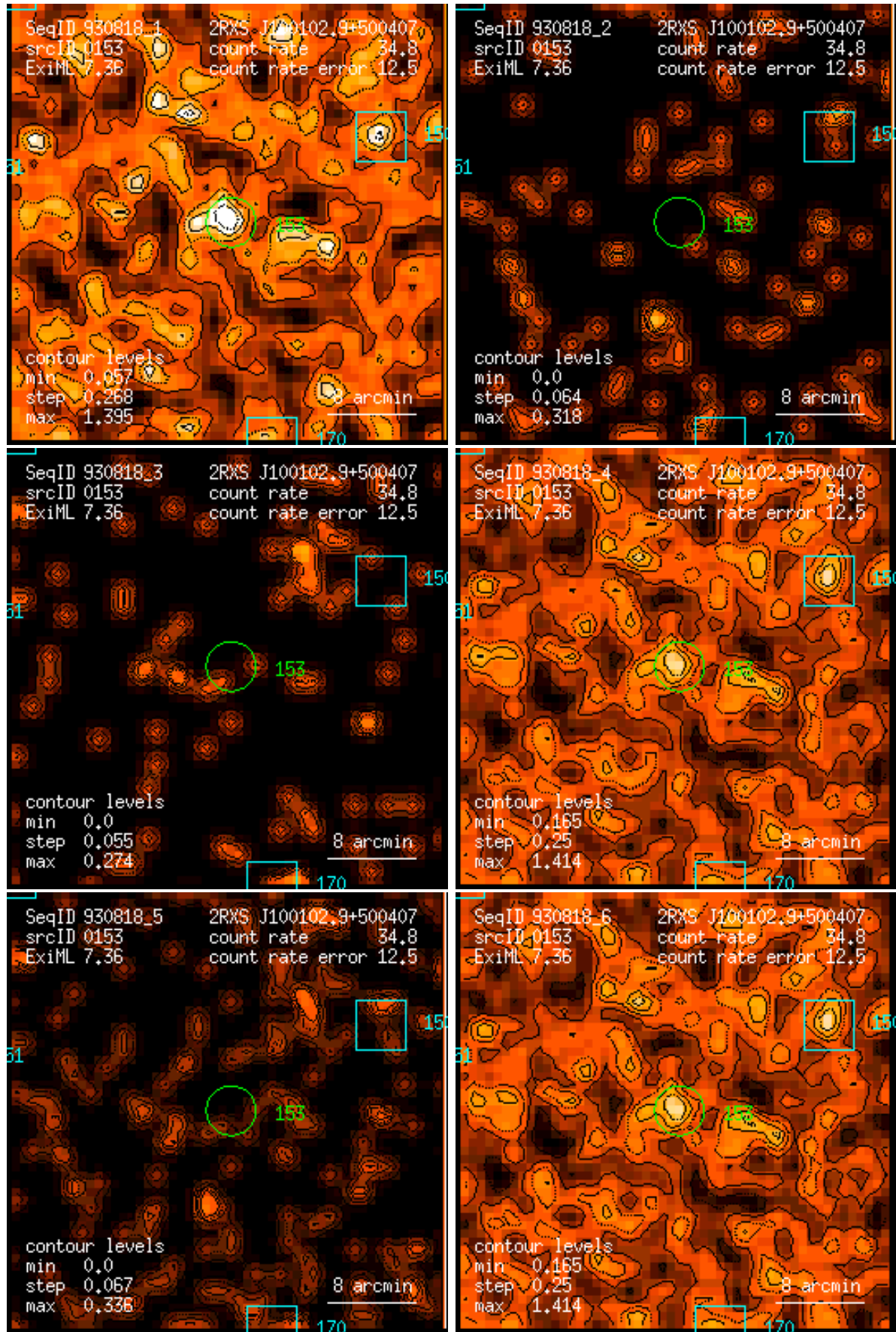
Figure 153: RASS 930818: detection 0153: band rate images, Gaussian filter: (1) PSPC channels 11 – 41, (2) 52 – 90, (3) 91 – 201, (4) 11 – 235, (5) 52 – 201, (6) 11 – 201. Broad band rates in counts/ks. Band rate contour levels in counts/ks/arcmin 2 .
