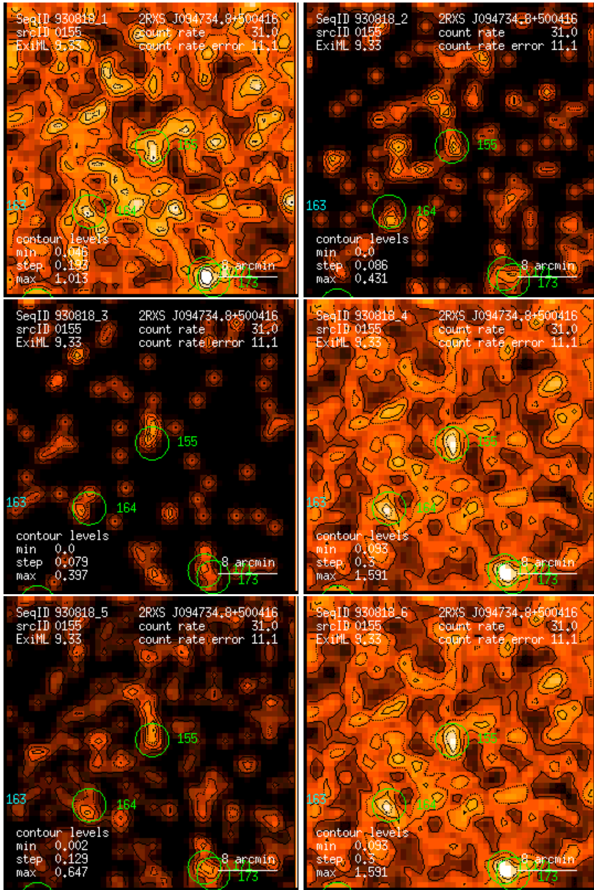
Figure 155: RASS 930818: detection 0155: band rate images, Gaussian filter: (1) PSPC channels 11 – 41, (2) 52 – 90, (3) 91 – 201, (4) 11 – 235, (5) 52 – 201, (6) 11 – 201. Broad band rates in counts/ks. Band rate contour levels in counts/ks/arcmin 2 .
