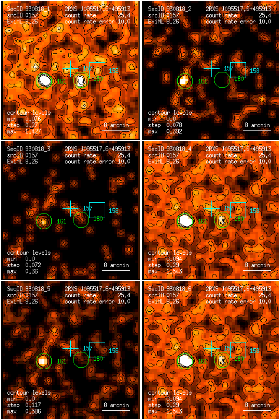
Figure 157: RASS 930818: detection 0157: band rate images, Gaussian filter: (1) PSPC channels 11 – 41, (2) 52 – 90, (3) 91 – 201, (4) 11 – 235, (5) 52 – 201, (6) 11 – 201. Broad band rates in counts/ks. Band rate contour levels in counts/ks/arcmin 2 .
