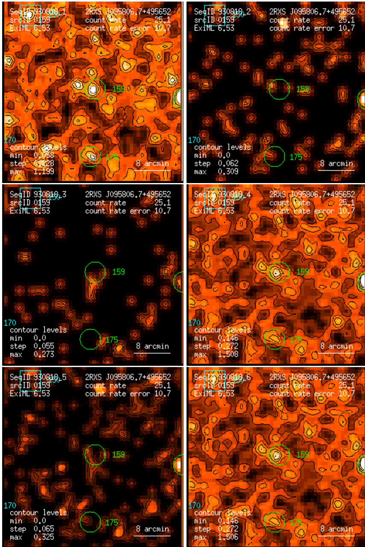
Figure 159: RASS 930818: detection 0159: band rate images, Gaussian filter: (1) PSPC channels 11 – 41, (2) 52 – 90, (3) 91 – 201, (4) 11 – 235, (5) 52 – 201, (6) 11 – 201. Broad band rates in counts/ks. Band rate contour levels in counts/ks/arcmin 2 .
