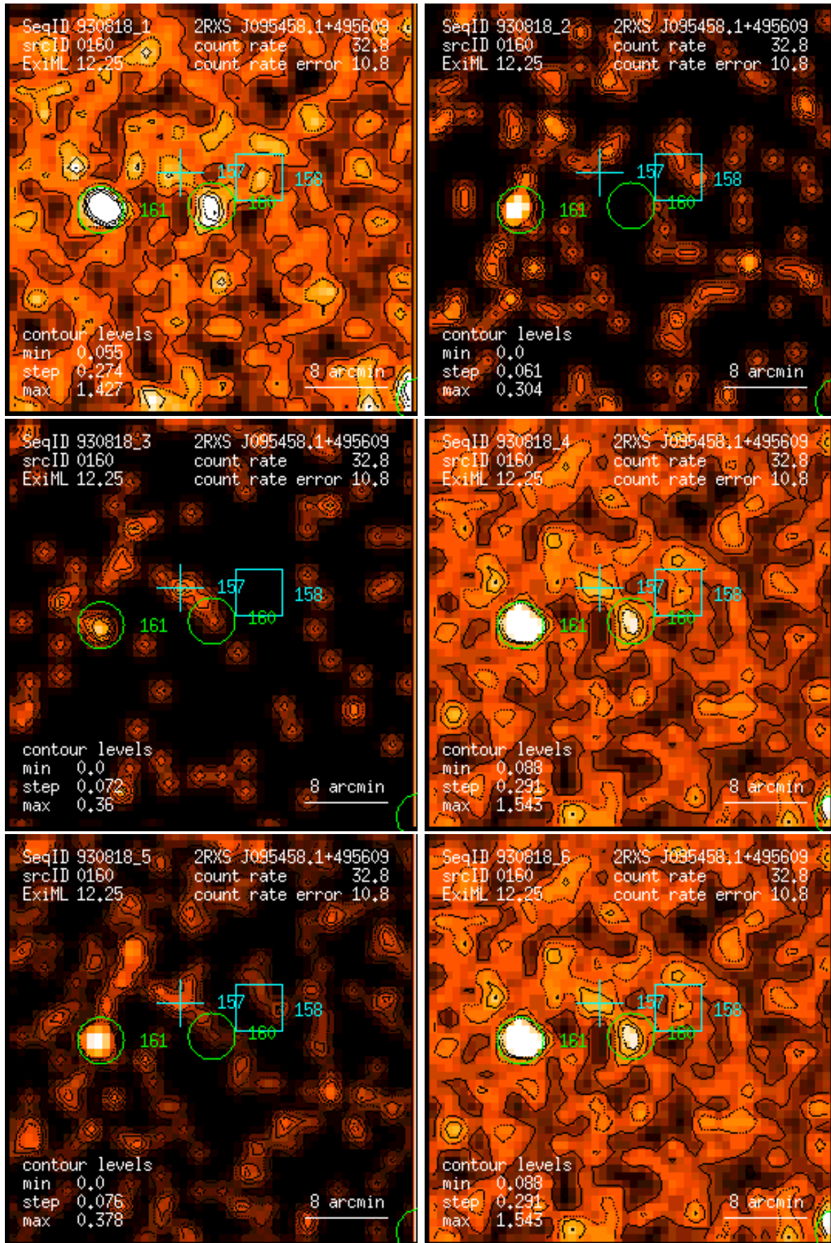
Figure 160: RASS 930818: detection 0160: band rate images, Gaussian filter: (1) PSPC channels 11 – 41, (2) 52 – 90, (3) 91 – 201, (4) 11 – 235, (5) 52 – 201, (6) 11 – 201. Broad band rates in counts/ks. Band rate contour levels in counts/ks/arcmin 2 .
