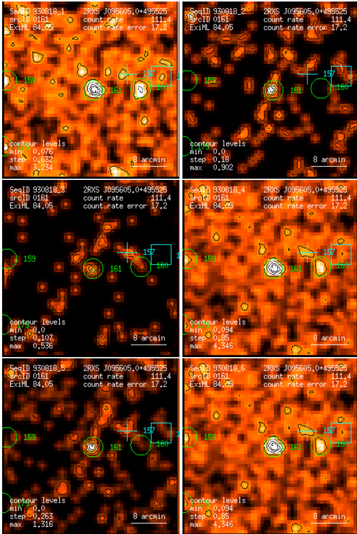
Figure 161: RASS 930818: detection 0161: band rate images, Gaussian filter: (1) PSPC channels 11 – 41, (2) 52 – 90, (3) 91 – 201, (4) 11 – 235, (5) 52 – 201, (6) 11 – 201. Broad band rates in counts/ks. Band rate contour levels in counts/ks/arcmin 2 .
