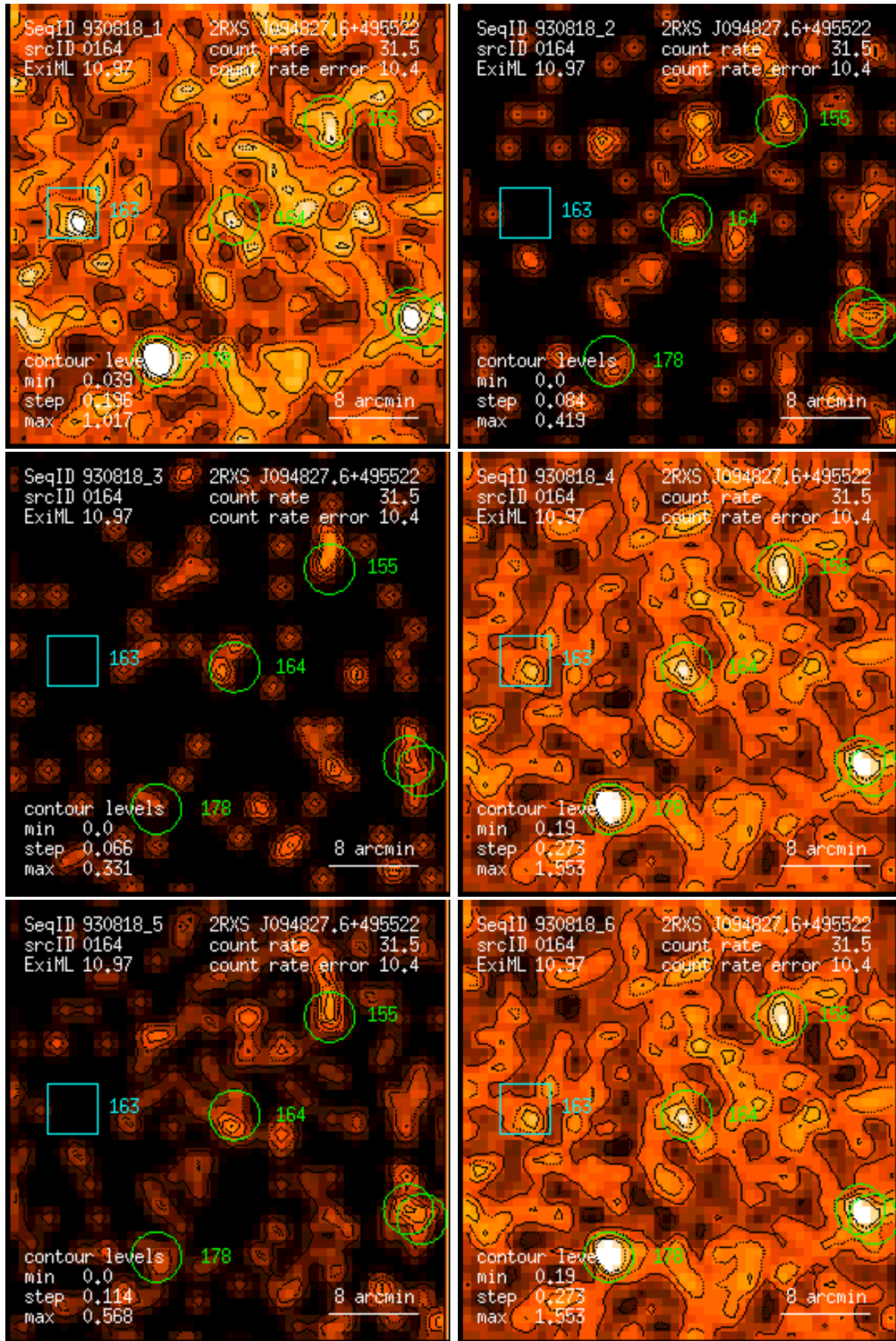
Figure 164: RASS 930818: detection 0164: band rate images, Gaussian filter: (1) PSPC channels 11 – 41, (2) 52 – 90, (3) 91 – 201, (4) 11 – 235, (5) 52 – 201, (6) 11 – 201. Broad band rates in counts/ks. Band rate contour levels in counts/ks/arcmin 2 .
