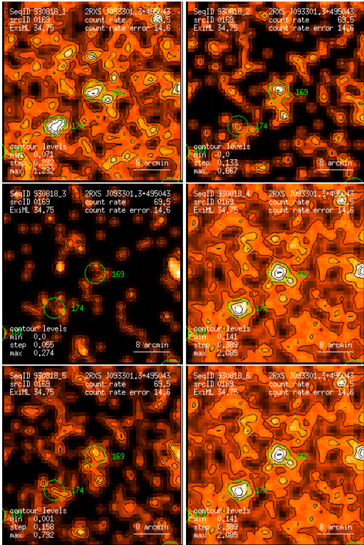
Figure 169: RASS 930818: detection 0169: band rate images, Gaussian filter: (1) PSPC channels 11 – 41, (2) 52 – 90, (3) 91 – 201, (4) 11 – 235, (5) 52 – 201, (6) 11 – 201. Broad band rates in counts/ks. Band rate contour levels in counts/ks/arcmin 2 .
