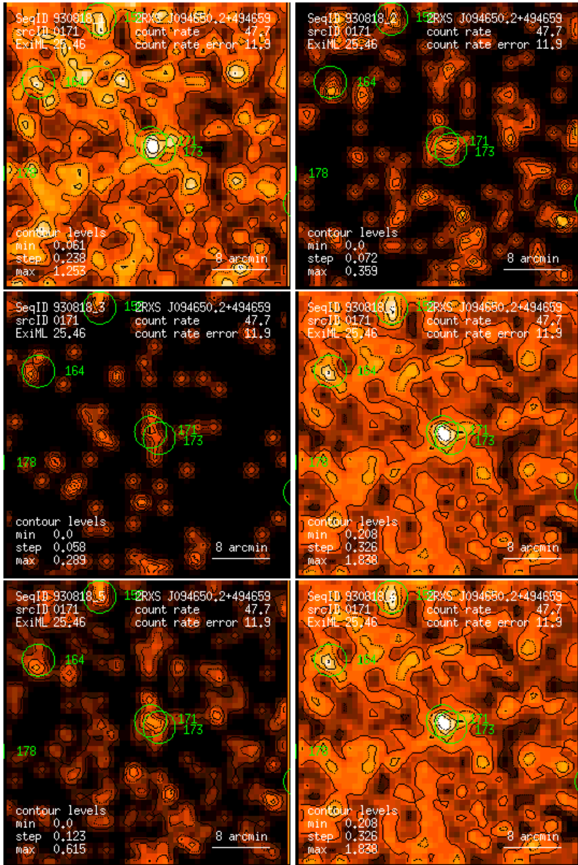
Figure 171: RASS 930818: detection 0171: band rate images, Gaussian filter: (1) PSPC channels 11 – 41, (2) 52 – 90, (3) 91 – 201, (4) 11 – 235, (5) 52 – 201, (6) 11 – 201. Broad band rates in counts/ks. Band rate contour levels in counts/ks/arcmin 2 .
