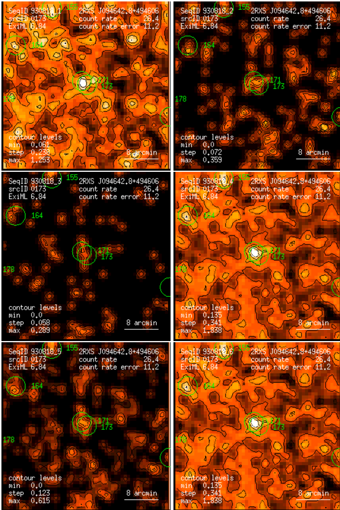
Figure 173: RASS 930818: detection 0173: band rate images, Gaussian filter: (1) PSPC channels 11 – 41, (2) 52 – 90, (3) 91 – 201, (4) 11 – 235, (5) 52 – 201, (6) 11 – 201. Broad band rates in counts/ks. Band rate contour levels in counts/ks/arcmin 2 .
