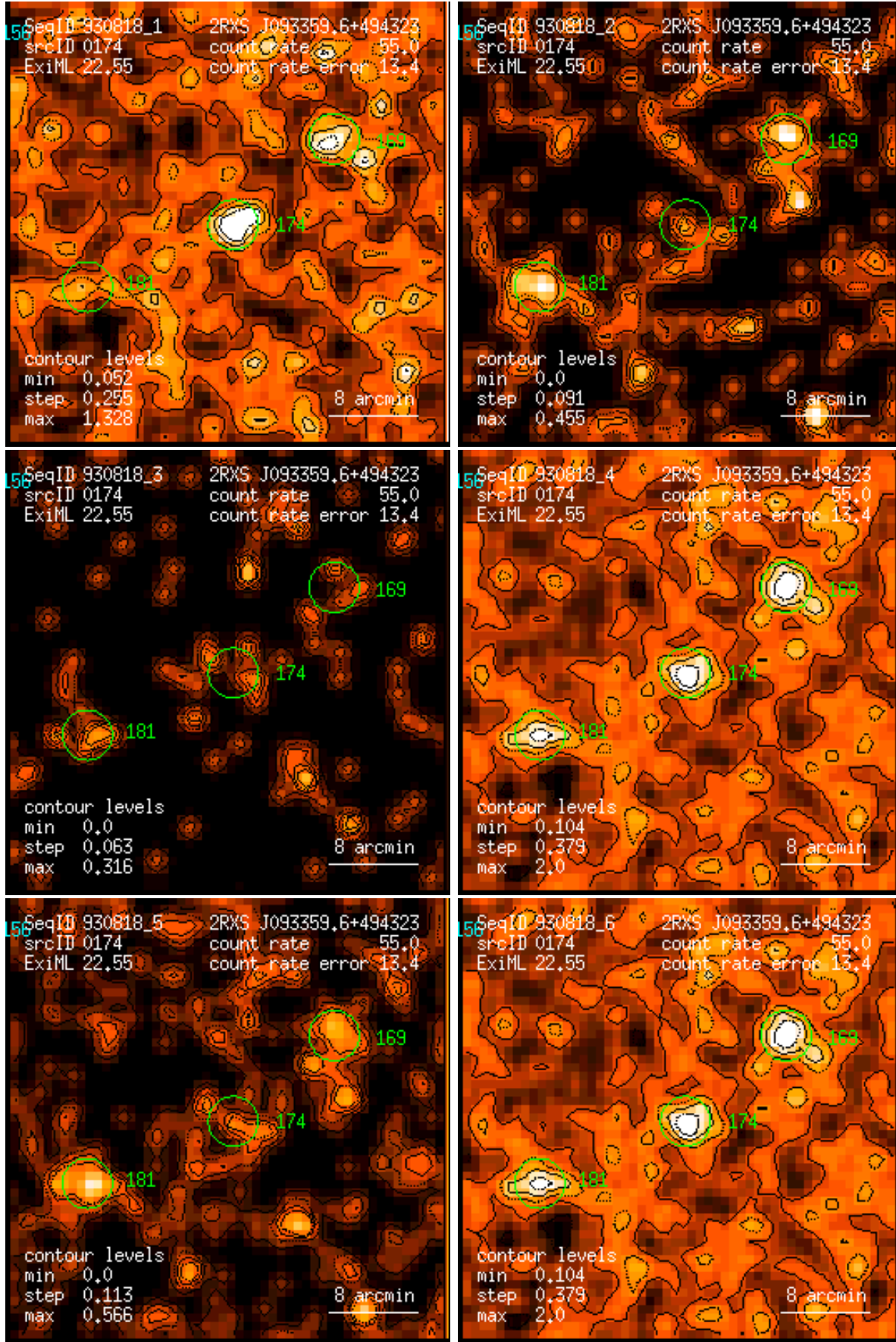
Figure 174: RASS 930818: detection 0174: band rate images, Gaussian filter: (1) PSPC channels 11 – 41, (2) 52 – 90, (3) 91 – 201, (4) 11 – 235, (5) 52 – 201, (6) 11 – 201. Broad band rates in counts/ks. Band rate contour levels in counts/ks/arcmin 2 .
