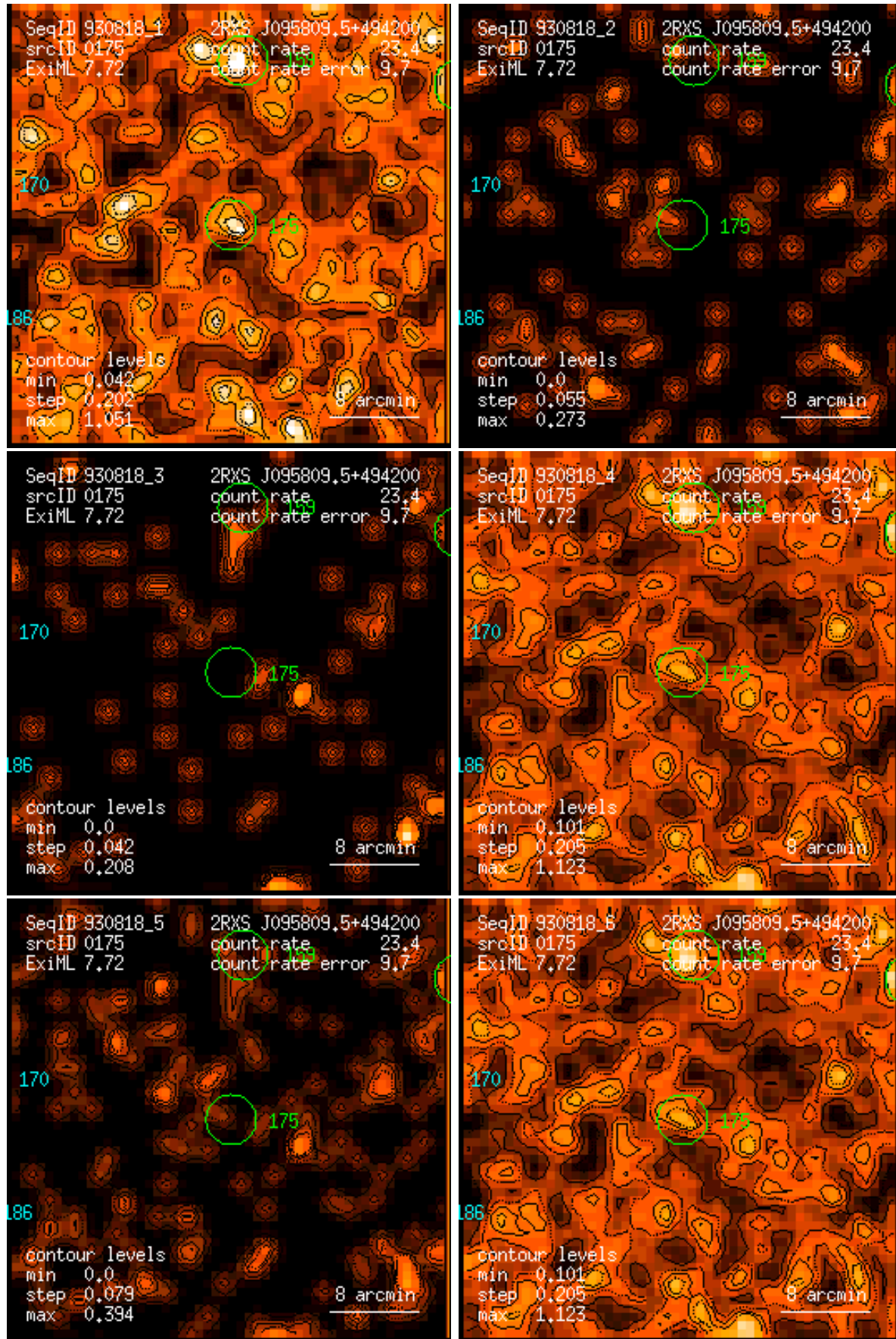
Figure 175: RASS 930818: detection 0175: band rate images, Gaussian filter: (1) PSPC channels 11 – 41, (2) 52 – 90, (3) 91 – 201, (4) 11 – 235, (5) 52 – 201, (6) 11 – 201. Broad band rates in counts/ks. Band rate contour levels in counts/ks/arcmin 2 .
