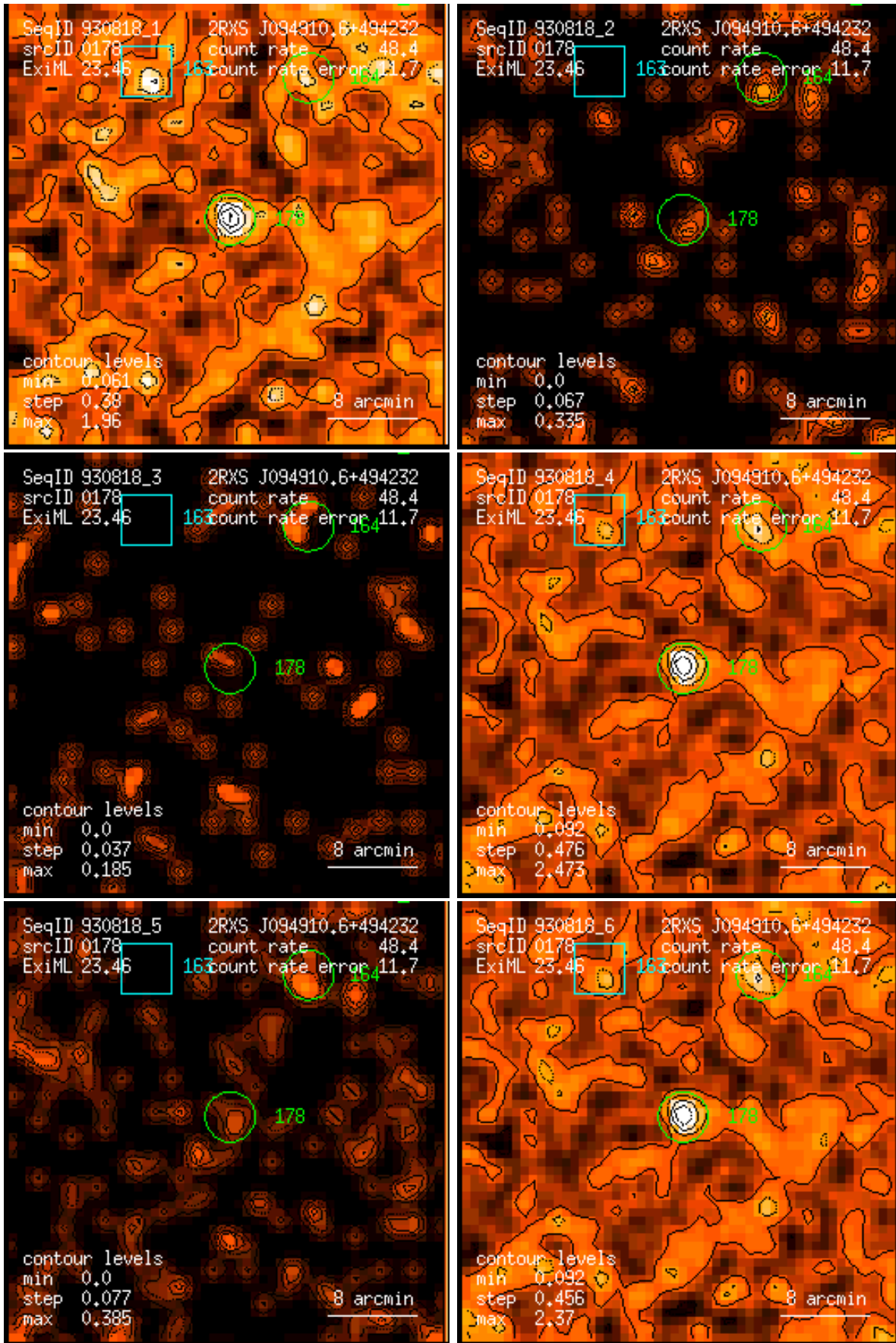
Figure 178: RASS 930818: detection 0178: band rate images, Gaussian filter: (1) PSPC channels 11 – 41, (2) 52 – 90, (3) 91 – 201, (4) 11 – 235, (5) 52 – 201, (6) 11 – 201. Broad band rates in counts/ks. Band rate contour levels in counts/ks/arcmin 2 .
