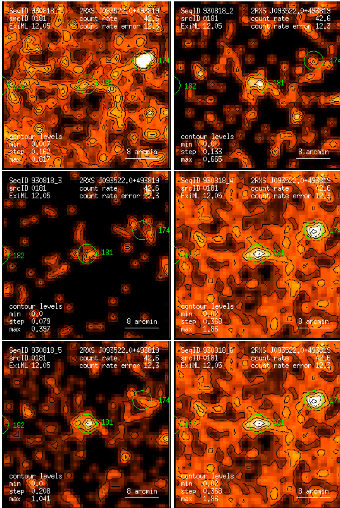
Figure 181: RASS 930818: detection 0181: band rate images, Gaussian filter: (1) PSPC channels 11 – 41, (2) 52 – 90, (3) 91 – 201, (4) 11 – 235, (5) 52 – 201, (6) 11 – 201. Broad band rates in counts/ks. Band rate contour levels in counts/ks/arcmin 2 .
