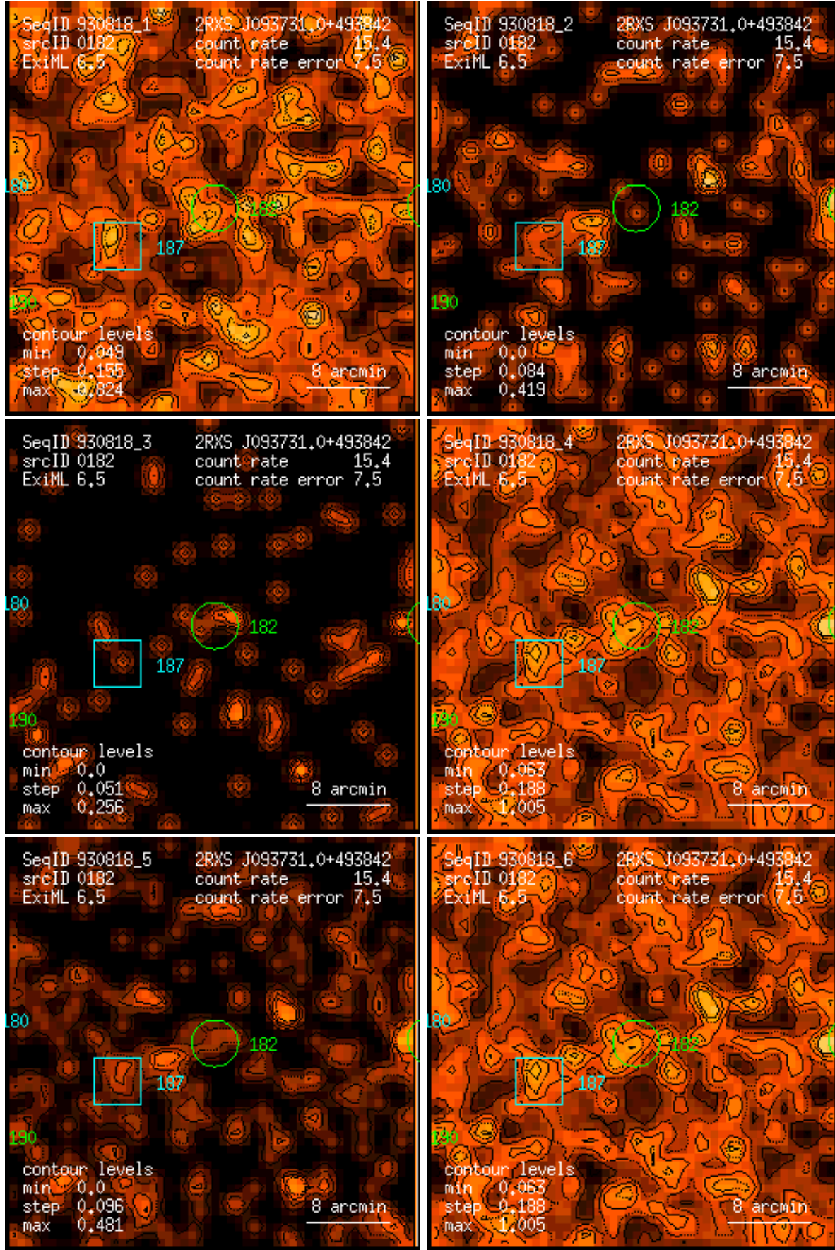
Figure 182: RASS 930818: detection 0182: band rate images, Gaussian filter: (1) PSPC channels 11 – 41, (2) 52 – 90, (3) 91 – 201, (4) 11 – 235, (5) 52 – 201, (6) 11 – 201. Broad band rates in counts/ks. Band rate contour levels in counts/ks/arcmin 2 .
