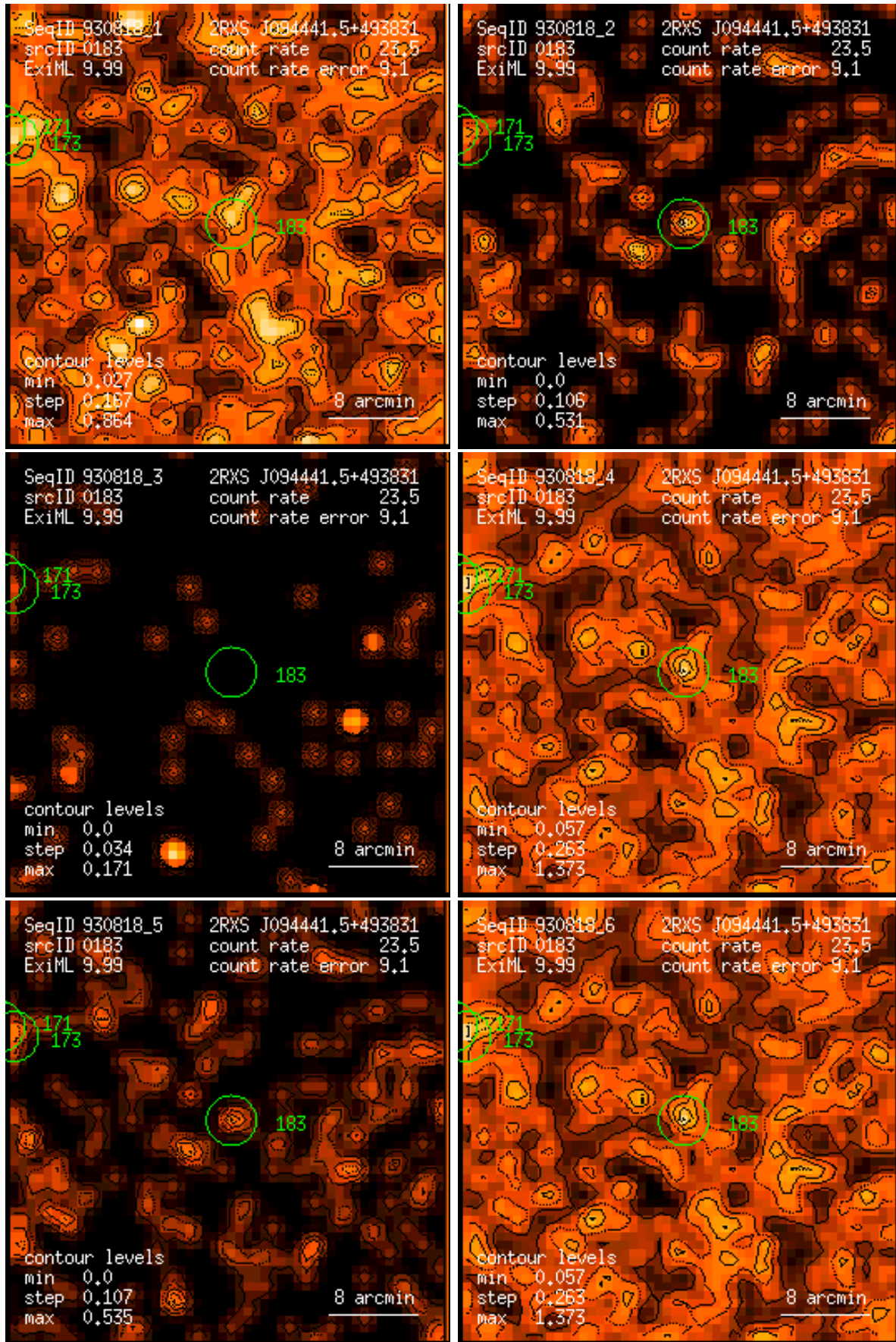
Figure 183: RASS 930818: detection 0183: band rate images, Gaussian filter: (1) PSPC channels 11 – 41, (2) 52 – 90, (3) 91 – 201, (4) 11 – 235, (5) 52 – 201, (6) 11 – 201. Broad band rates in counts/ks. Band rate contour levels in counts/ks/arcmin 2 .
