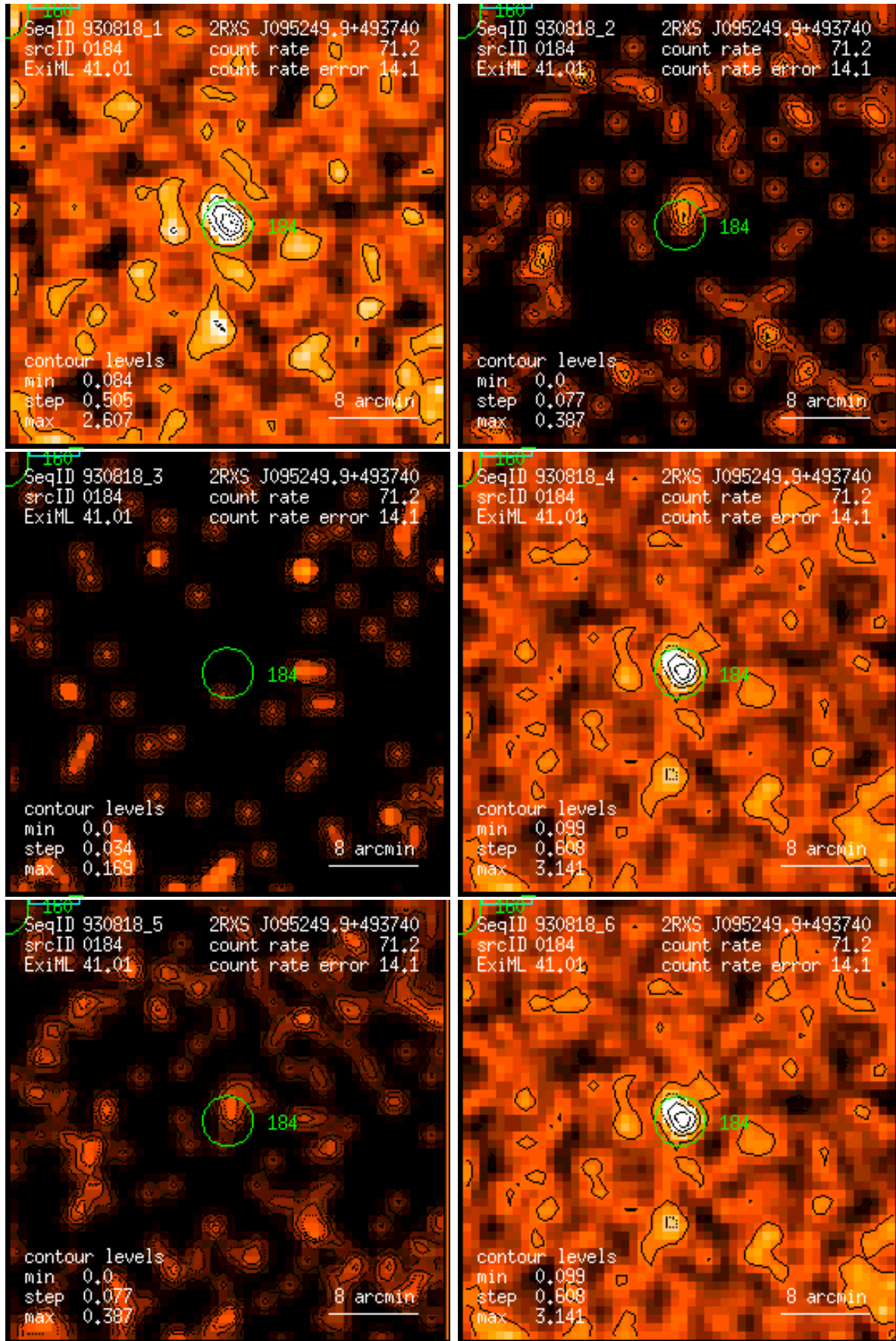
Figure 184: RASS 930818: detection 0184: band rate images, Gaussian filter: (1) PSPC channels 11 – 41, (2) 52 – 90, (3) 91 – 201, (4) 11 – 235, (5) 52 – 201, (6) 11 – 201. Broad band rates in counts/ks. Band rate contour levels in counts/ks/arcmin 2 .
