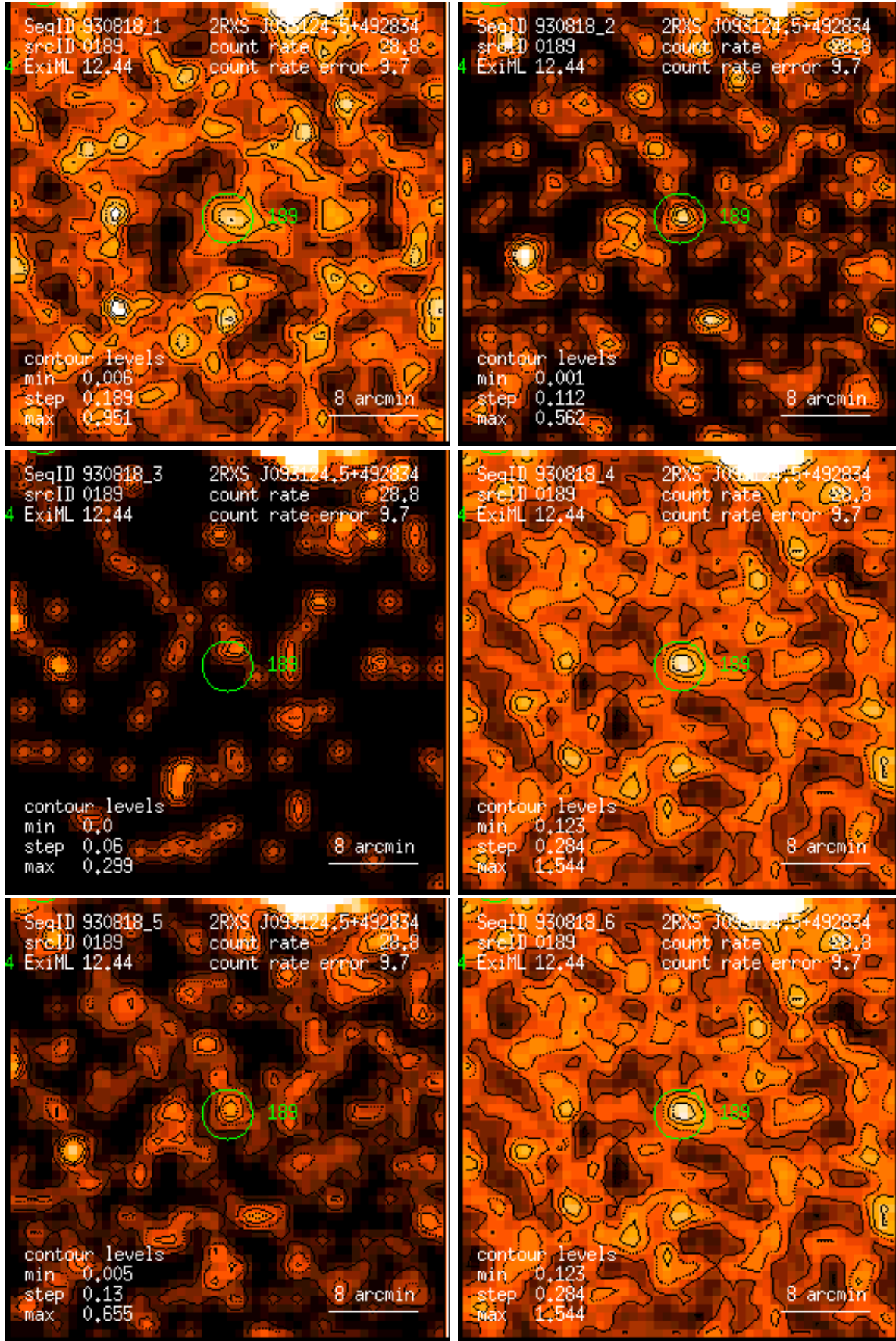
Figure 189: RASS 930818: detection 0189: band rate images, Gaussian filter: (1) PSPC channels 11 – 41, (2) 52 – 90, (3) 91 – 201, (4) 11 – 235, (5) 52 – 201, (6) 11 – 201. Broad band rates in counts/ks. Band rate contour levels in counts/ks/arcmin 2 .
